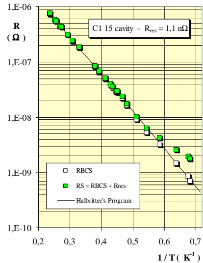
Figure 2 : R_S vs. He bath temperature (before cavity baking).
