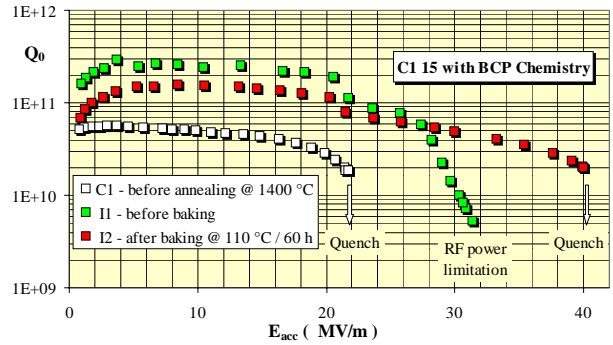
Figure 1 : Q_0(E_{\text{acc}}) curves for the C1-15 BCP cavity, the best result is performed after annealing and baking.
