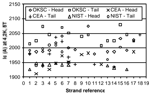
Fig. 11. Strand critical currents cross checks
