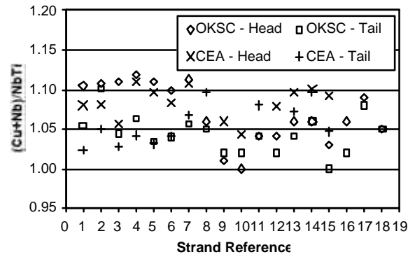
Fig. 12. (Cu+Nb)/NbTi cross checks
