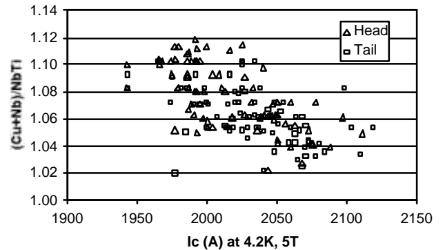
Fig. 8. (\text{Cu+Nb})/\text{NbTi} ratio versus critical current, data from Outokumpu.
