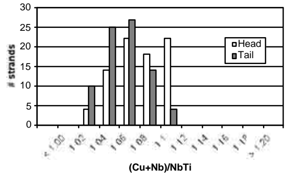
Fig. 7. (\text{Cu+Nb})/\text{NbTi} ratio at both strand ends, data from Outokumpu.
