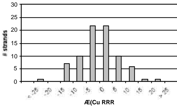
Fig. 10. Cu RRR difference: Tail - Head, data from Outokumpu.
