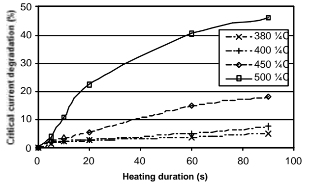
Fig. 14. I_c degradation at 5 T vs. heating duration at various temperature
