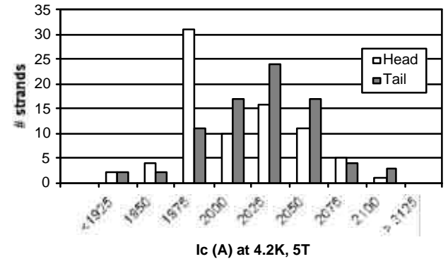
Fig. 3. Critical currents at both strand ends, data from Outokumpu.
