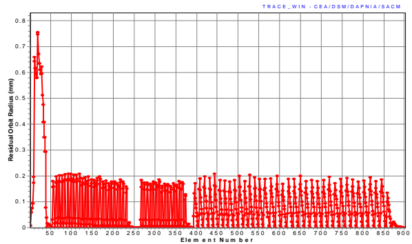
Figure 6: rms residual orbit with both H^- and H^+
