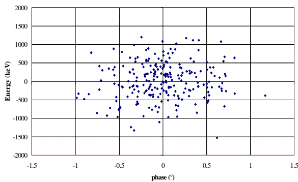
Figure 5: Position of the beam c.o.g. in longitudinal phase-space at linac exit for different error sets.
