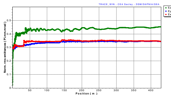
Figure 1: H^- beam rms emittances growth.
