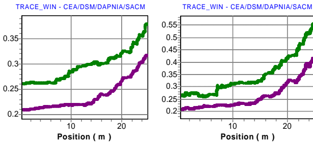
Figure 4: Transverse (violet) and longitudinal (green) rms emittance growths in envelope (left) and multiparticle simulation (right).
