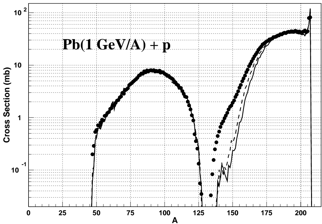
Fig 3: Cross section of spallation residues produced by Au + p at 800 MeV per nucleon (top) 8) and by Pb + p at 1 GeV per nucleon (bottom) 7) as a function of their atomic mass (A). Data points are compared to the INCL4+ABLA calculation without (continuous lines) and with (dashed lines) emission of light clusters in the cascade.
