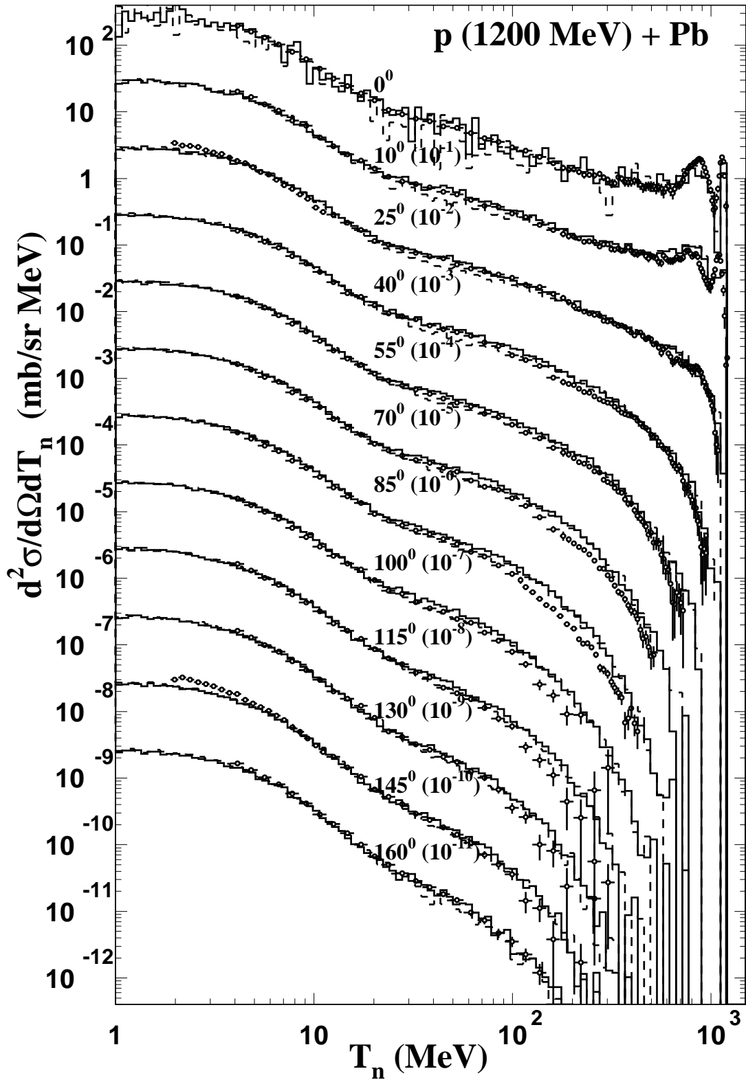
Fig. 1. Neutron production double differential cross sections from proton on lead at 1.2 GeV. Data from 3) are the points, INCL4+ABLA calculations are histograms without (continuous lines) and with (dashed lines) emission of light clusters in the cascade. Cross sections are properly normalized for the smallest angle; for the others they are divided by successive powers of ten as indicated.
