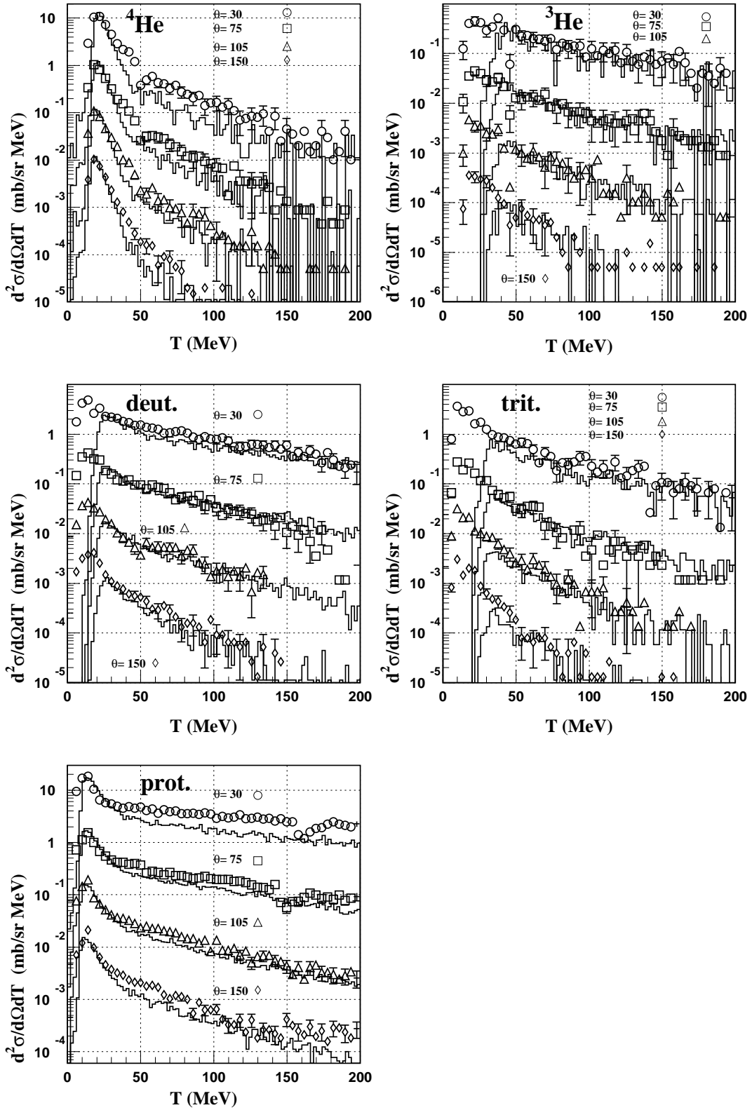
Fig 5: Double differential cross sections of protons and light composites produced in the p (2.5 GeV) +Au interaction and measured by the NESSI collaboration 10) are compared with the INCL4+ABLA calculation (histograms) including the production of composites in the cascade. Only the {}^4\text{He} composite is emitted by the evaporation code ABLA. Data are displayed with the same convention as in Fig 1.
