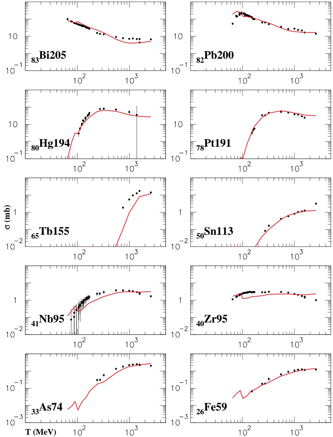
Fig. 4. Cross sections in mb for the production of residual nuclei for the p+Pb system as a function of the proton incident energy in MeV. Data points are from ref 9) . Lines are the INCL4-ABLA results.
