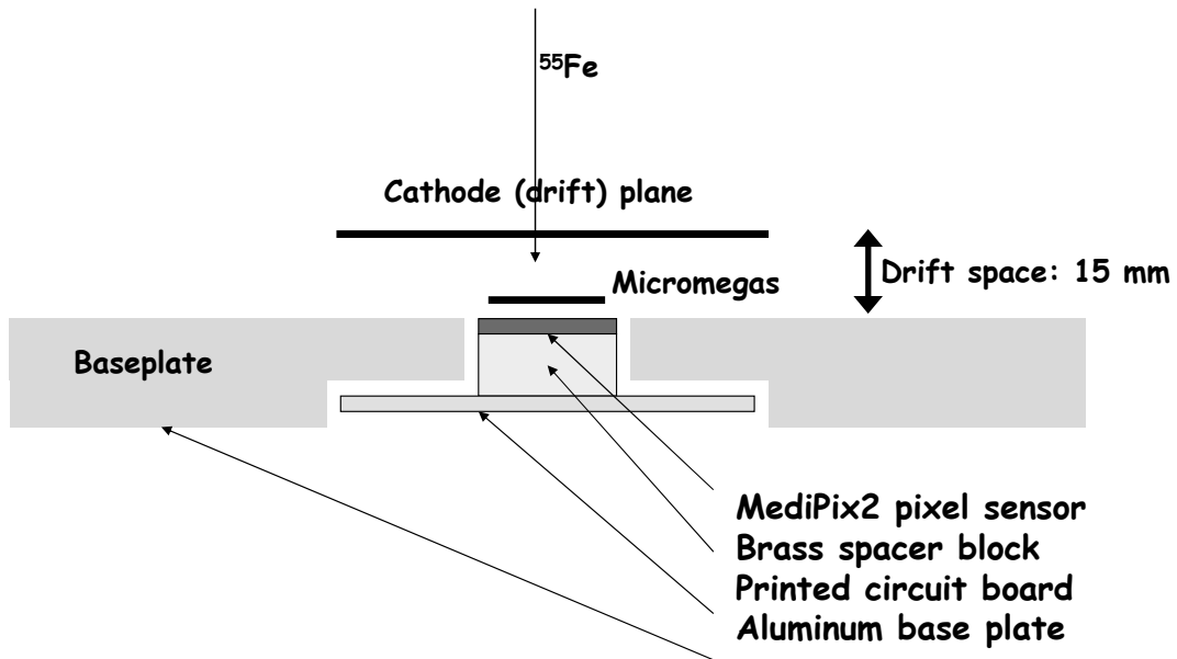
Fig. 2. The layout of the chamber with the MediPix2, the Micromegas and the drift gap.
