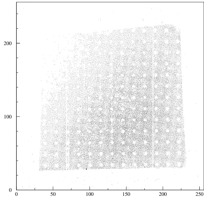
Fig. 11. Superimposed images recorded from the MediPix2/Micromegas prototype TPC after irradiation with \beta 's from a ^{90}\text{Sr} source.
