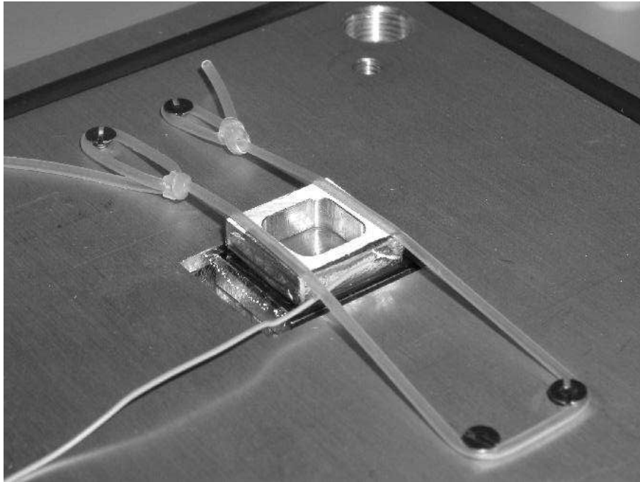
Fig. 3. The mounting of the Micromegas onto the MediPix2 sensor.
