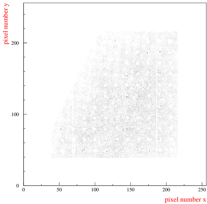
Fig. 14. Superimposed images recorded with a modified MediPix2 sensor during one night of cosmics data taking.
