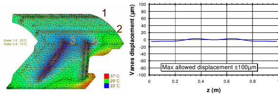
Figure 5 : Temperatures and vane displacement
