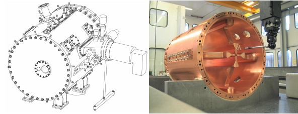
Figure 3 : SPIRAL 2 RFQ prototype cavity
