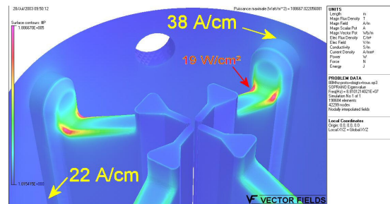
Figure 4: 3D view of the power deposition
