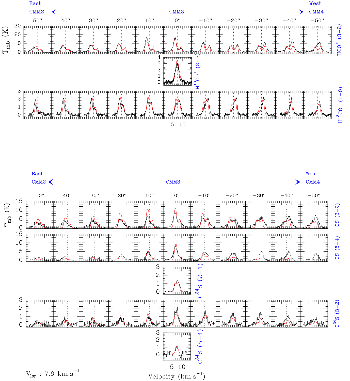
Fig. 10. \text{HCO}^+ (3-2) , \text{H}^{13}\text{CO}^+ (3-2) , \text{H}^{13}\text{CO}^+ (1-0) (top) and \text{CS} (3-2) , \text{CS} (5-4) , \text{C}^{34}\text{S} (2-1) , \text{C}^{34}\text{S} (3-2) , \text{C}^{34}\text{S} (5-4) (bottom) spectra observed along an East-West axis going through C-MM2, C-MM3, C-MM4 in NGC 2264-C. Synthetic spectra corresponding to the “best-fit” 2D radiative transfer model described in the text (see Fig. 8c for input parameters) are superimposed in light grey. The central position corresponds to C-MM3.
