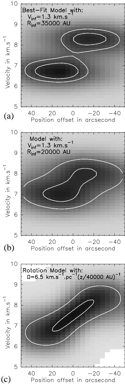
Fig. 12. Synthetic \text{H}^{13}\text{CO}^+ (1-0) position-velocity diagrams calculated for three different radiative transfer models. a) Diagram corresponding to the ‘best-fit’ model (see text for details). b) Diagram obtained by changing R_{\text{inf}} to 20000 AU. c) Diagram obtained for a bulk (differential) rotation of the model cloud about an axis centered on C-MM3 and perpendicular to the line joining C-MM2, C-MM3, and C-MM4. These diagrams have to be compared with the observed \text{H}^{13}\text{CO}^+ (1-0) diagram shown at the top right of Fig. 6.
