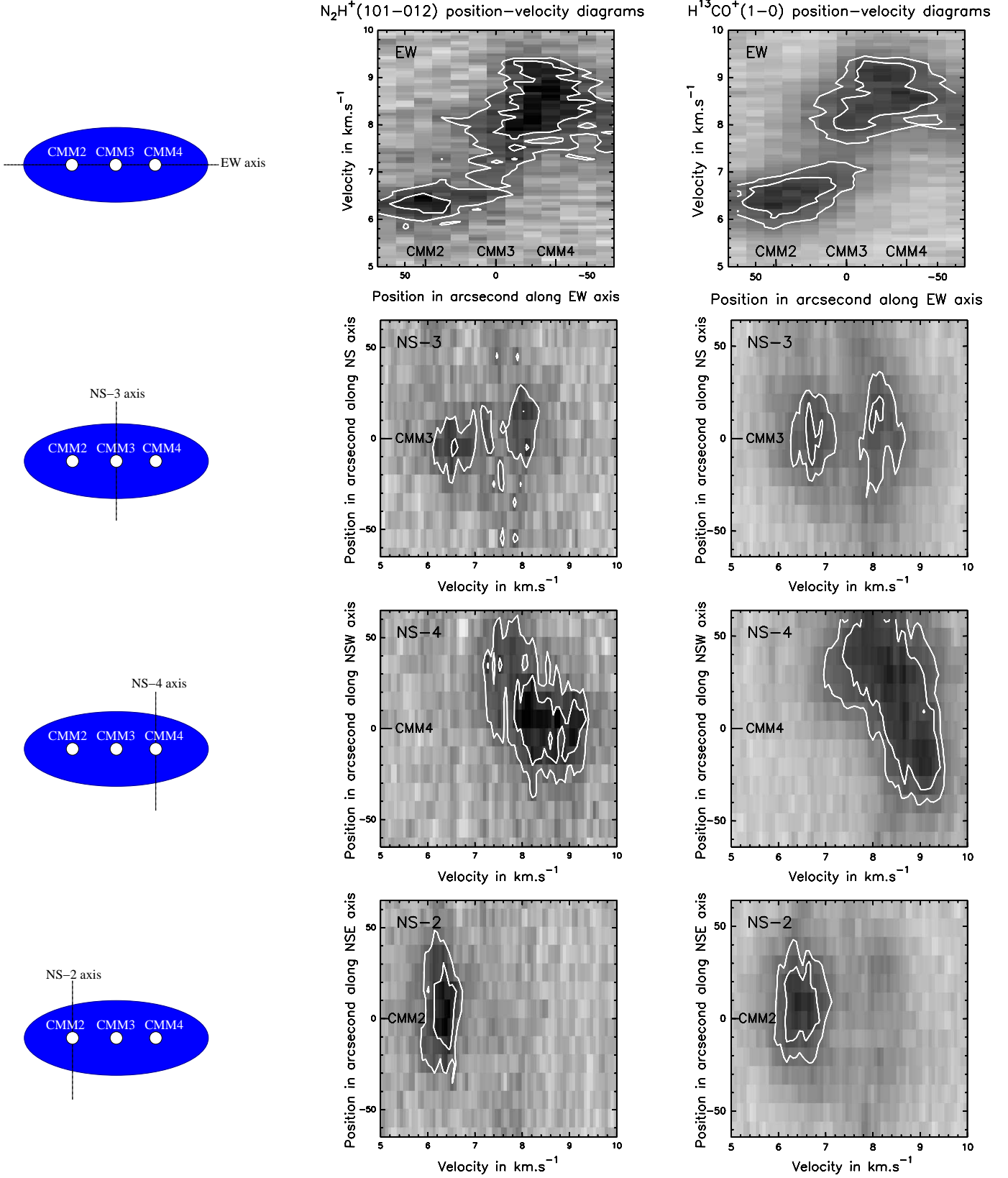
Fig. 6. N_2H^+(101-012) and H^{13}CO^+(1-0) position-velocity diagrams observed in the central part of NGC 2264-C along four axes shown schematically on the left. From top to bottom: the first row corresponds to PV diagrams taken along an East-West (EW) axis going through C-MM2, C-MM3, and C-MM4; the second row corresponds to a North-South axis going through C-MM3 (NS-3); the third row is for a North-South axis going through C-MM4 (NS-4); the fourth row is for a North-South axis going through C-MM2 (NS-2). Contour levels are 1.1 and 1.8 K for the N_2H^+(101-012) diagrams, 1.05 and 1.4 K for the H^{13}CO^+(1-0) diagrams.
