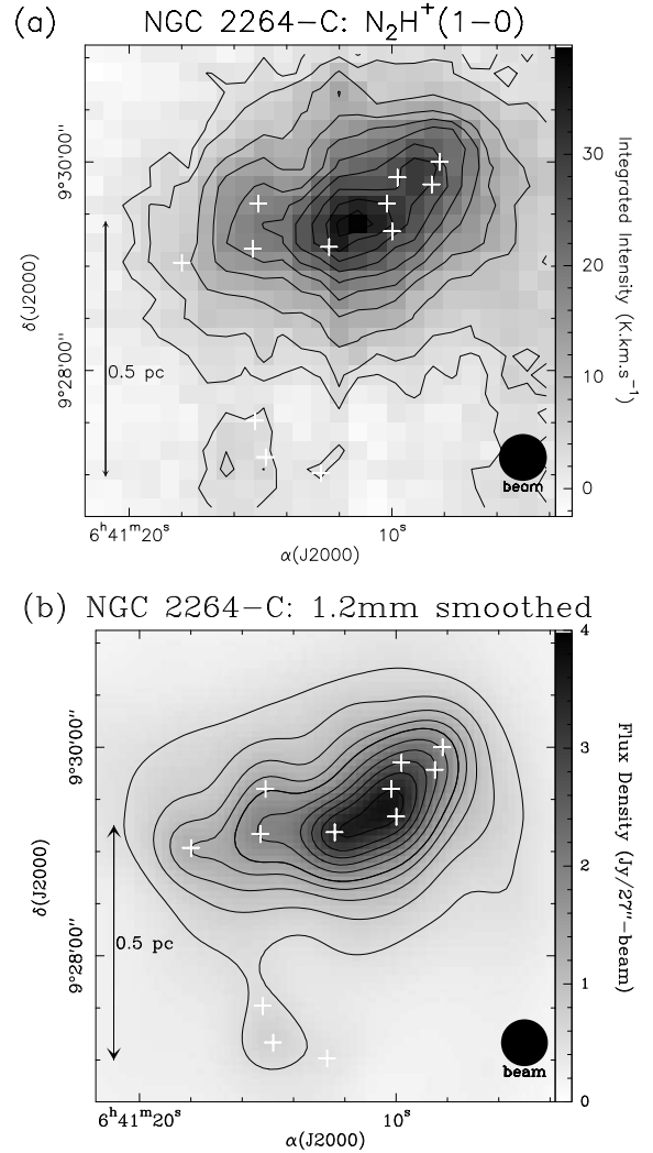
Fig. 4. a) Map of the N_2H^+(1-0) integrated line intensity from 0 to 25 \text{ km.s}^{-1} in NGC 2264-C. First contour at 2 \text{ K.km.s}^{-1} ; other contours go from 4 to 36 \text{ K.km.s}^{-1} by 4 \text{ K.km.s}^{-1} . b) Millimeter dust continuum map of NGC 2264-C smoothed to the same 27'' (HPBW) angular resolution as the N_2H^+(1-0) map. Contour levels go from 0.5 to 1.5 \text{ Jy}/27''\text{-beam} by 0.25 \text{ Jy}/27''\text{-beam} and from 1.5 to 3 \text{ Jy}/27''\text{-beam} by 0.375 \text{ Jy}/27''\text{-beam} . The white crosses mark the positions of the millimeter continuum sources identified in § 3.
