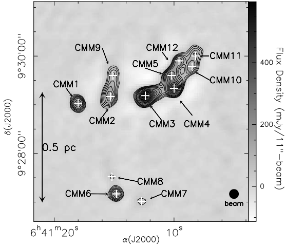
(b) NGC 2264-C: 1.2mm filtered
