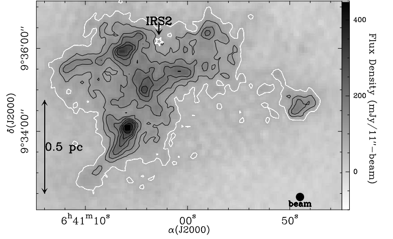
(b) NGC 2264-D: 1.2mm filtered
