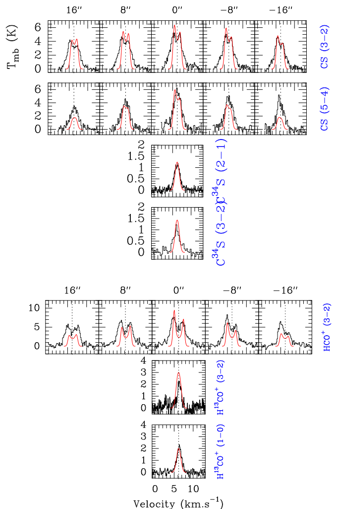
Fig. 14. CS(3-2), CS(5-4), \text{C}^{34}\text{S}(2-1) , \text{C}^{34}\text{S}(3-2) (top), and \text{HCO}^+(3-2) , \text{H}^{13}\text{CO}^+(3-2) , \text{H}^{13}\text{CO}^+(1-0) (bottom) spectra observed along the direction of maximum velocity gradient (P.A. grad \sim +45^\circ ) through D-MM1. Synthetic spectra corresponding to the “best-fit” 2D radiative transfer model described in the text are superimposed in light grey. Positive offsets are located to the North-East of D-MM1, while negative offsets are to the South-West.
