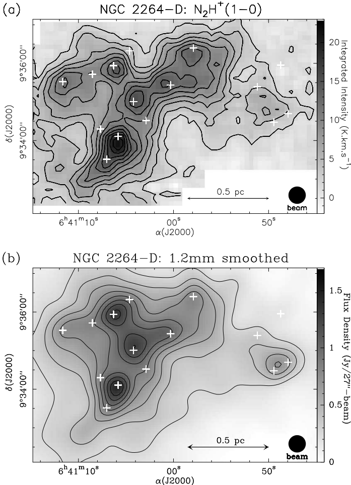
Fig. 5. Same as Fig. 4 for NGC 2264-D. a) Contour levels go from 2 to 20 \text{K.km.s}^{-1} by 2 \text{K.km.s}^{-1} . b) Contour levels go from 0.25 to 1.3 \text{Jy}/27''\text{-beam} by 0.15 \text{Jy}/27''\text{-beam} .
