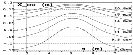
Figure 3: Closed orbits at various energies.
