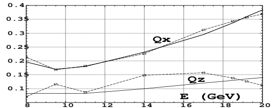
Figure 4: Cell tunes vs. energy obtained either from matrix method or (markers) from ray-tracing.
