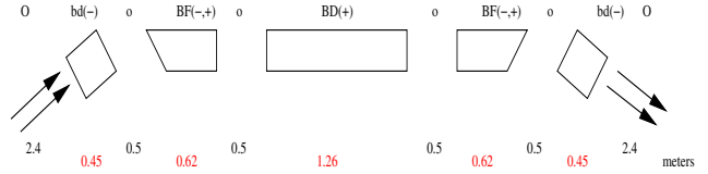
Figure 1: Isochronous cell.
