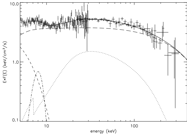
Fig. 9. Epoch 4 unabsorbed EF(E) spectrum of Cygnus X-1 along with the best-fit model described in Table 2 with the JEM-X, IBIS/ISGRI and SPI data. Dashed: Disc. Dotted: Gaussian line. Dotted: Reflection. Long Dashes: Comptonization. Thick: Total model.
