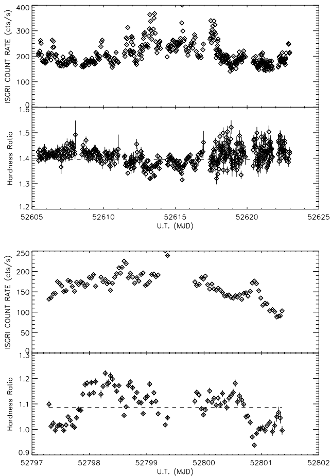
Fig. 3. Top: Zoom on the 20–200 keV IBIS/ISGRI light curve of Cygnus X-1 from 2002 November 25 until December 15 and corresponding HR between the 40–100 and the 20–30 keV energy bands (average level denoted by dashed line). Bottom: Same as above for epoch 2.
