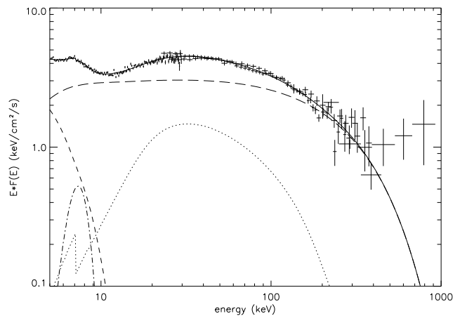
Fig. 7. Epoch 2 unabsorbed EF(E) spectrum of Cygnus X-1 along with the best-fit model described in Table 2 with the JEM-X, SPI and IBIS (ISGRI and PICsIT) data. Dashed: Disc. Dotted-Dashed: Gaussian line. Dotted: Reflection. Long Dashes: Comptonization. Thick: Total model.
