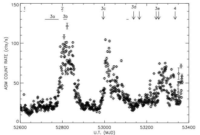
Fig. 1. RXTE / ASM daily average (1.5–12 keV) light curve of Cygnus X-1 from 2002 November to 2004 November (MJD = JD – 2400000.5) with the periods of our INTEGRAL observations (see text and Tables 1 and 2 for epoch definitions).
