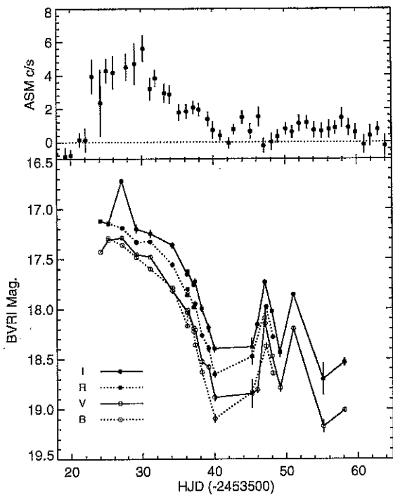
Figure 2. RXTE ASM light curve for SAX J1808.4-3658 (upper panel) and BVRI band light curves (lower panel).
