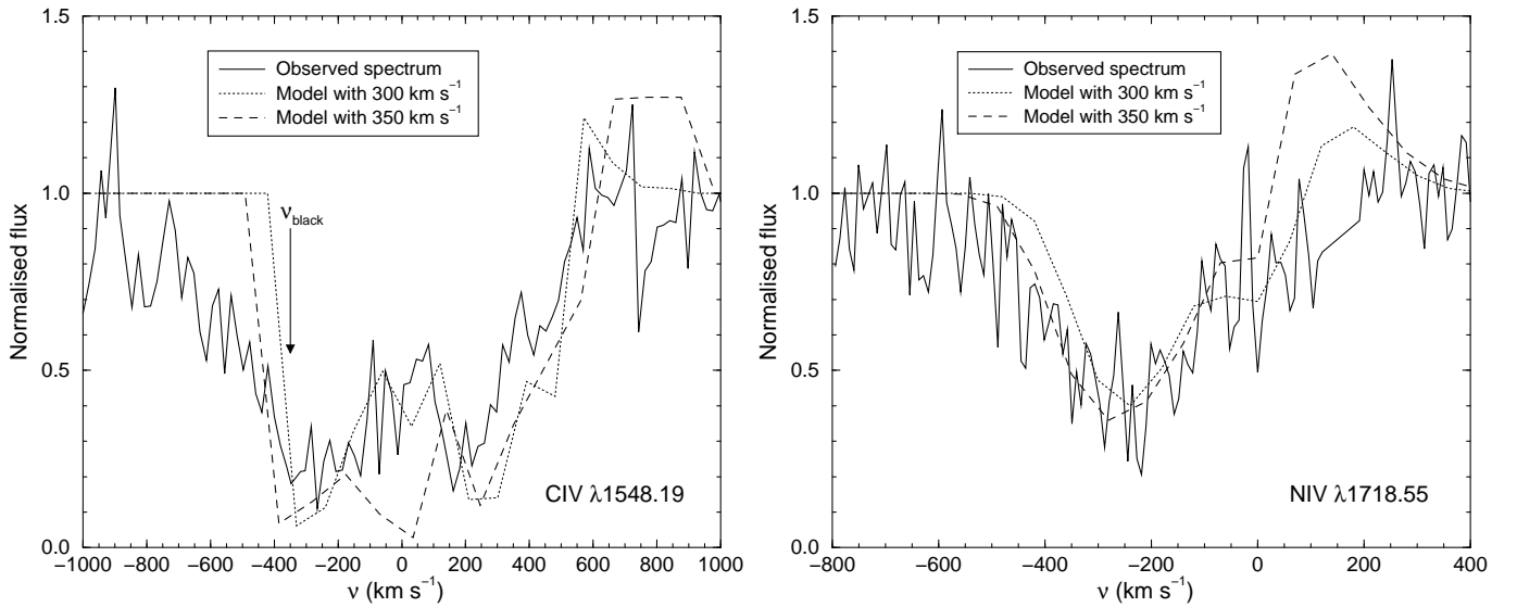
Fig. 1. Profiles of the observed UV doublet C iv \lambda\lambda 1548.19–1550.76 (left panel, where v = 0 \text{ km s}^{-1} corresponds to the blue line of the doublet) and the line N iv \lambda 1718.55 (right panel) with the theoretical models for 300 and 350 \text{km s}^{-1} superimposed to them. The arrow in the left plot indicates v_{\text{black}} = 350 \text{ km s}^{-1} . The wind terminal velocity is clearly slower than 500 \text{km s}^{-1} .
