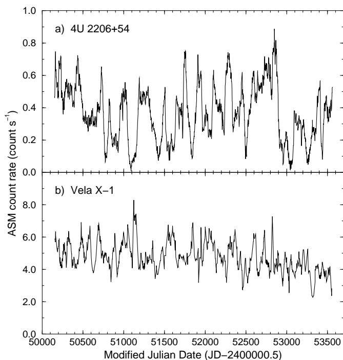
Fig. 3. a) The data shown in Fig. 2 smoothed with a running window of 30 days of length, allowing a much better visualisation of the long-term flux variability. b) The same procedure applied to the RXTE /ASM data of the wind-fed HMXB Vela X-1 (after excluding the data taken during its X-ray eclipses). Recurrent ups and downs are seen in both lightcurves.
