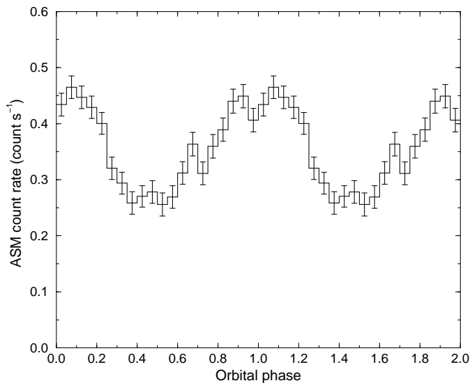
Fig. 7. DBD lightcurve of 4U 2206+54 folded using P_{\text{orb}}=9.5591 d and t_0=\text{MJD } 51856.6 . Error bars represent the error of the weighted mean in each of the 20 bin per period, and not the standard deviation. Two orbital periods are shown for clarity. A quasi-sinusoidal pattern is evident.
