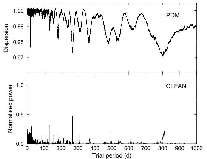
Fig. 4. Periodograms of the 10D-ODA lightcurve of 4U 2206+54 obtained by using the PDM (top) and CLEAN (bottom) algorithms. Apart from the \sim 9.6 d orbital period, a trial period around 270 d is clearly detected by both methods.
