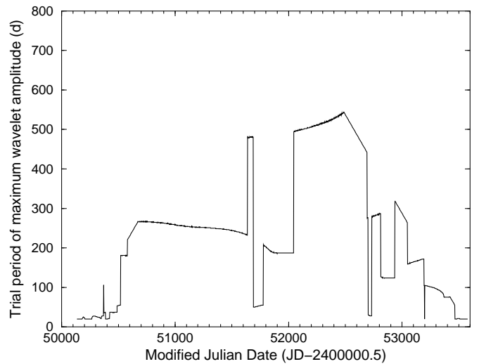
Fig. 6. Maxima of the wavelet amplitude map shown in Fig. 5 versus time for the 10D-ODA lightcurve of 4U 2206+54. The decrease of the quasi-period, with superimposed jumps, is clearly seen.
