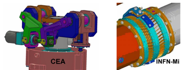
Figure 4: Design of two piezo-electric tuner prototypes
