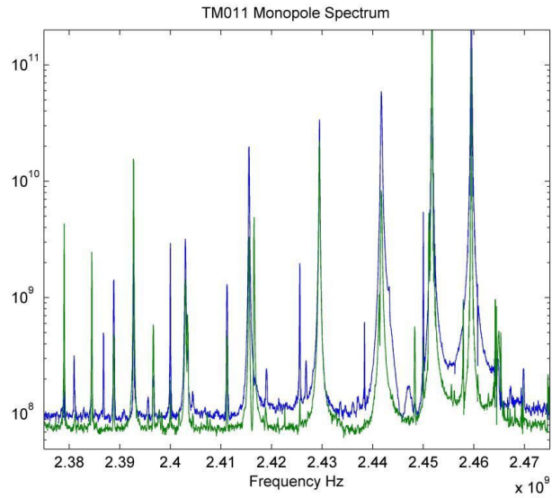
Figure 1. Monopole Spectrum, both couplers
