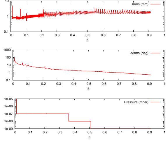
Figure 2: Evolution of the rms beam size in the transverse and longitudinal plane and the pressure of the residual gas in the ESS linac.
