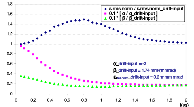
Figure 7: Relative evolution of the twiss parameter in a drift during the transient for a H^+ beam with 100 mA, 95keV, 4.10^{-5} hPa.
