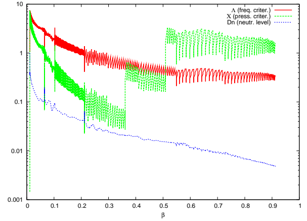
Figure 3: Behaviour of the neutralization level, the frequency criterion \Lambda and the pressure criterion \chi in the ESS linac.
