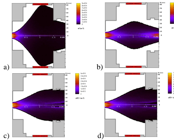
Figure 11: Distribution for the protons at 1\mu s in a), at 6\mu s in b), for the H_2^+ in c) and the H_3^+ in d) at the equilibrium.
