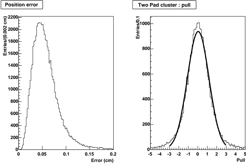
Fig. 6. Left plot: the estimated error distribution associated to clusters with two pads for B=0.2 T. The mean value of the distribution is 570 \mu\text{m} . Right plot: the pull of the cluster position with respect to the fit position of the track. The curve represents a gaussian fit to the distribution with a width of 1.1.
