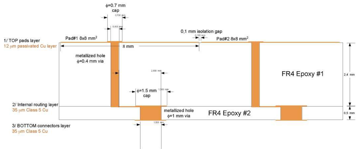
Fig. 2. The PCB cross-section.
