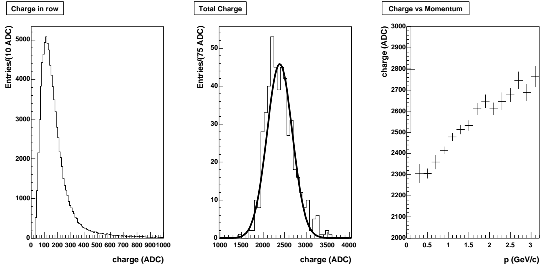
Fig. 9. Left plot: the charge per pad row. Middle plot: the 80% truncated mean for the sum of the charge in the two detectors. A resolution of 12.2% has been obtained. Right Plot: the measured charge versus the track momentum.
