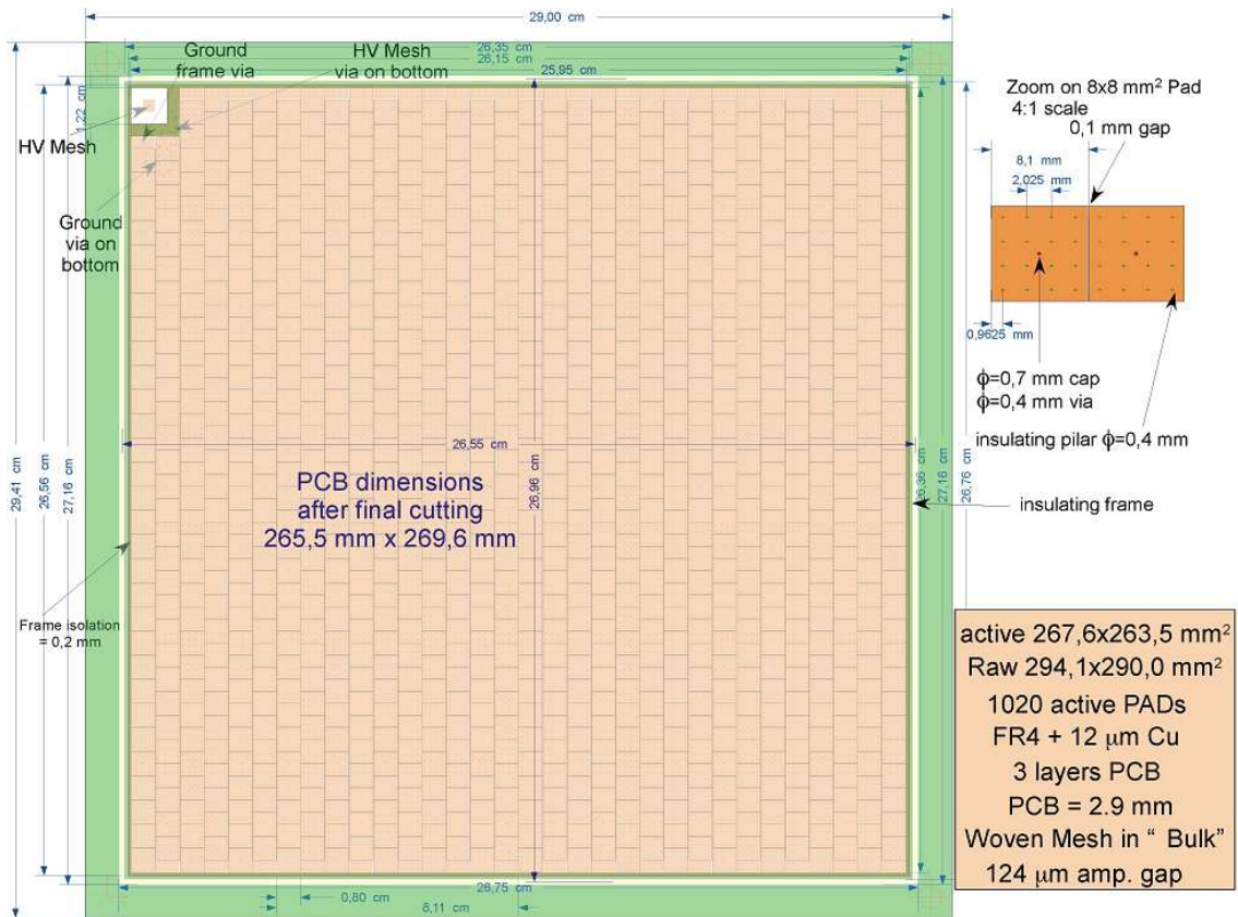
Fig. 1. View of the PCB from the anode pads side.
