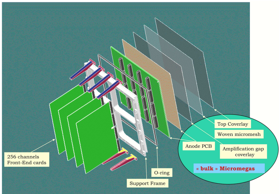
Fig. 3. Exploded 3D view of a Micromegas Module.
