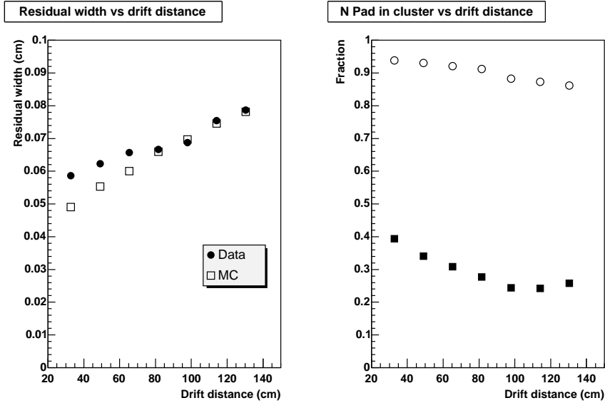
Fig. 7. Left plot: the gaussian width for the two pad cluster track residual as a function of the drift distance for B=0.2 T. The open squares show the width estimated using a Geant4 MC simulation. Right plot: the cumulative fraction of clusters with one pad (squares) and two pads (open circles).
