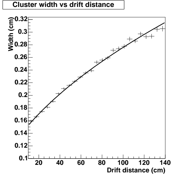
Fig. 8. Gaussian width of the electron cloud measured using the track position and the charge ratio in clusters with two pads as a function of the drift distance for B=0.2 T. The curve shows the result of the fit to the function \sqrt{s_0^2 + C_T l_{drift}} where the transverse diffusion coefficient C_T has been found 253 \mu\text{m}/\sqrt{\text{cm}} .
