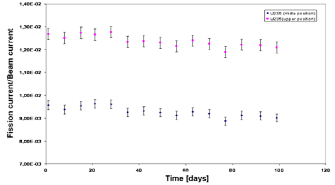
Fig. 4. Time evolution of the ^{235}\text{U} fission chamber signal, normalised to the proton beam current.
