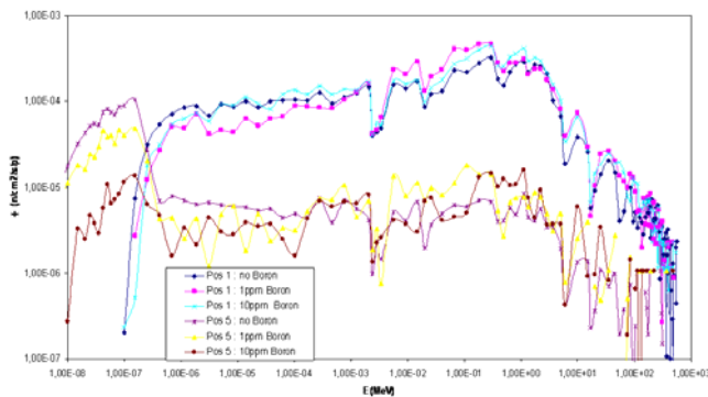
Fig. 6. Neutron energy distribution at the lower (Pos 1) and upper (Pos 5) position, obtained using no Boron, 1 ppm and 10 ppm Boron in the LBE composition.
