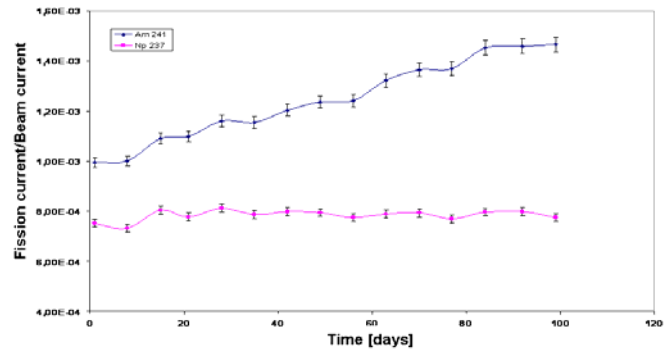
Fig. 5. Time evolution of the ^{241}\text{Am} and ^{237}\text{Np} fission chamber signal, normalised to the proton beam current.
