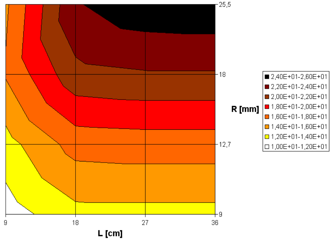
Figure 91: ^{206}\text{Hg} production rate per incident proton [ 10^{-6} \text{ s}^{-1} ] as a function of target radius R and length L , (target = Pb, E = 0.5 GeV, model = CEM2k, the low energetic secondary neutron flux is taken into account, CINDER evolution time = 1 ms).
