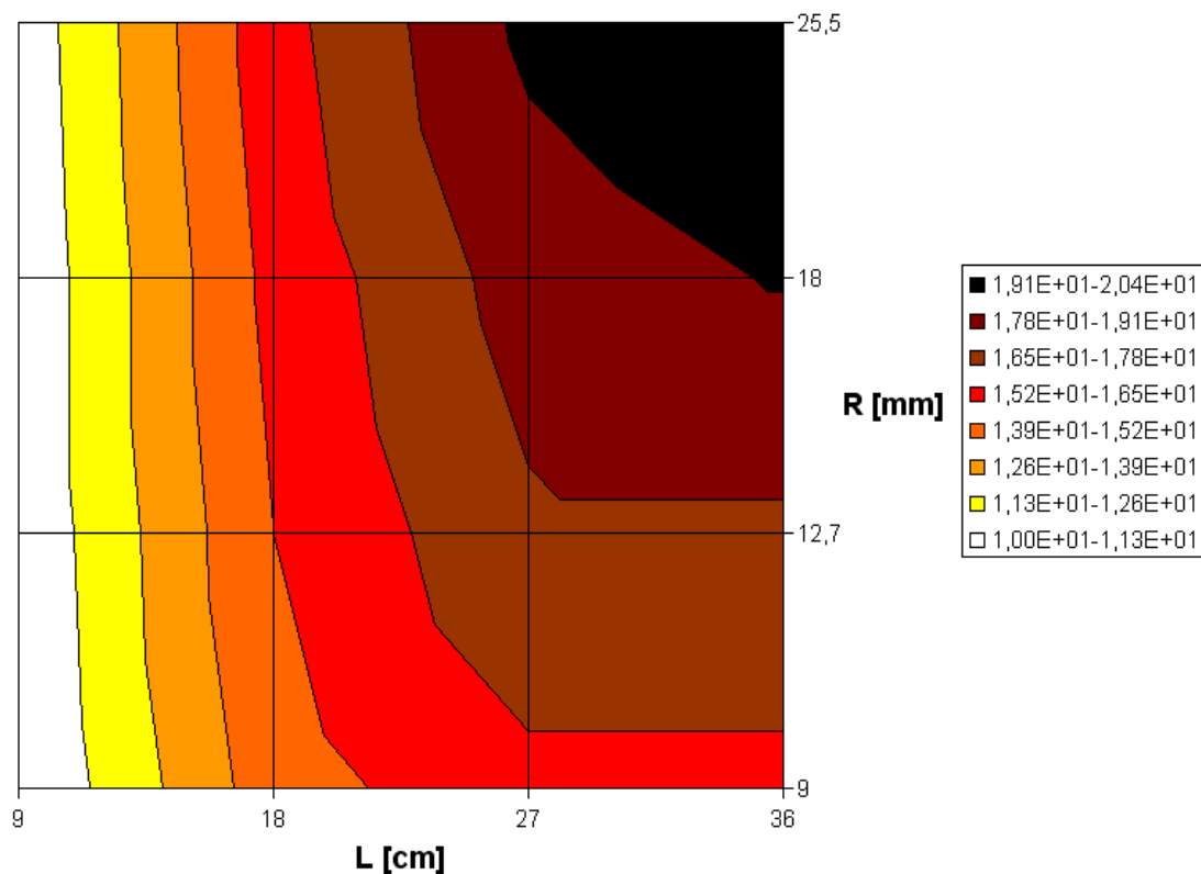
Figure 89: ^{180}\text{Hg} production rate per incident proton [ 10^{-6} \text{ s}^{-1} ] as a function of target radius R and length L , (target = Pb, E = 1 \text{ GeV} , model = CEM2k, the low energetic secondary neutron flux is taken into account, CINDER evolution time = 1 ms).
