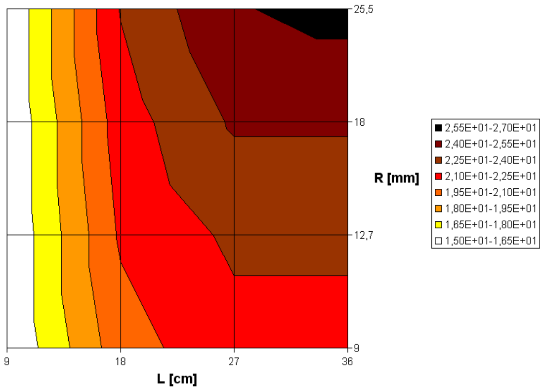
Figure 88: ^{180}\text{Hg} production rate per incident proton [ 10^{-6} \text{ s}^{-1} ] as a function of target radius R and length L , (target = Pb, E = 1 \text{ GeV} , model = INCL4/ABLA, the low energetic secondary neutron flux is taken into account, CINDER evolution time = 1 ms).
