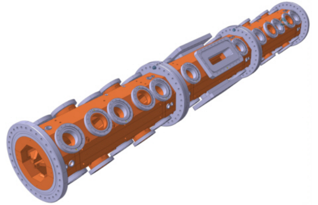
Figure 2: Linac4 RFQ.
