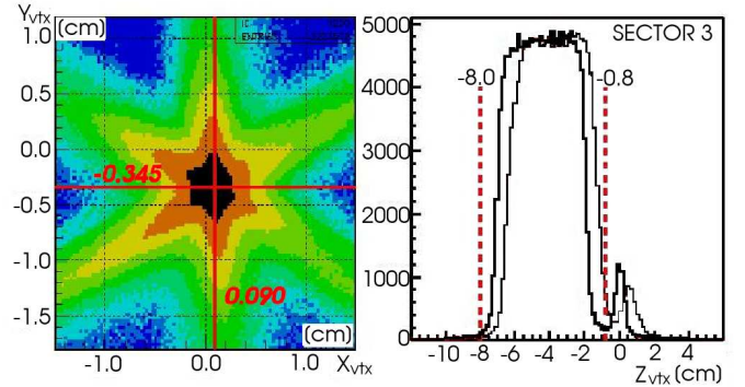
FIG. 5: (Color online) Left: Reconstructed x and y target positions, showing an offset of x=0.90 mm and y=-3.45 mm, respectively. The right panel shows the z -vertex before (thin solid line) and after (bold solid line) the beam offsets in the x and y target positions have been corrected.
