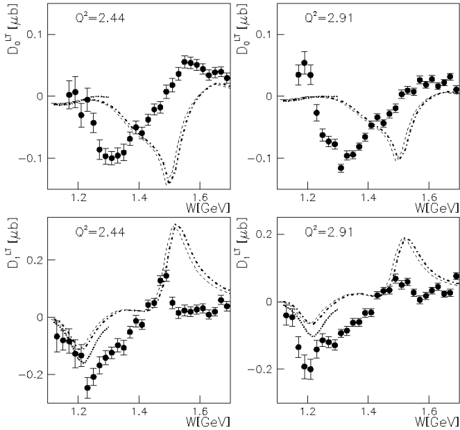
FIG. 24: Legendre moments D_0^{LT} (top) and D_1^{LT} (bottom) of structure function \sigma_{LT} . Curves as in Fig. 21.
