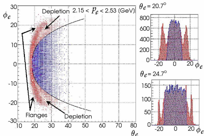
FIG. 8: (Color online) Electron fiducial cut at electron momentum range : 2.15 < p_e < 2.53 GeV for sector 1. The histograms on the right show the \phi_e distributions at two values of \theta_e . The highlighted area in the center indicates the selected fiducial range.
