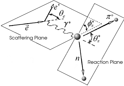
FIG. 1: Kinematics of single \pi^+ electroproduction.
