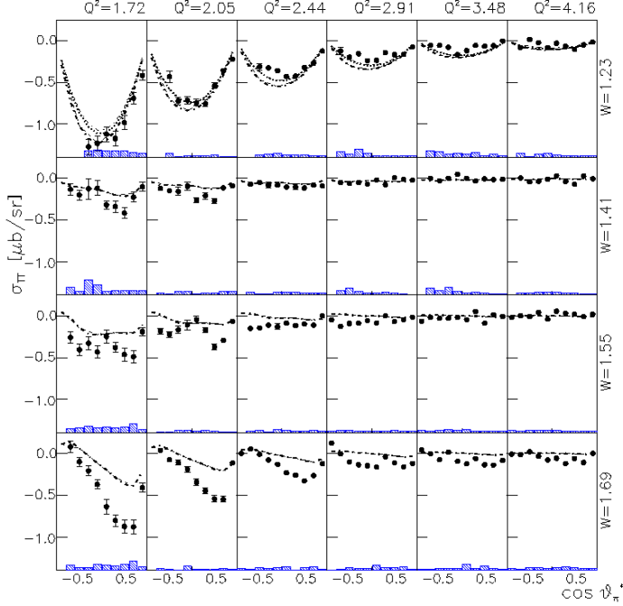
FIG. 17: Structure function \sigma_{TT} as a function of \cos \theta_\pi^* at fixed W and Q^2 compared to model calculations. Curves as in Fig. 15. Systematic uncertainties are shown in shaded bars.
