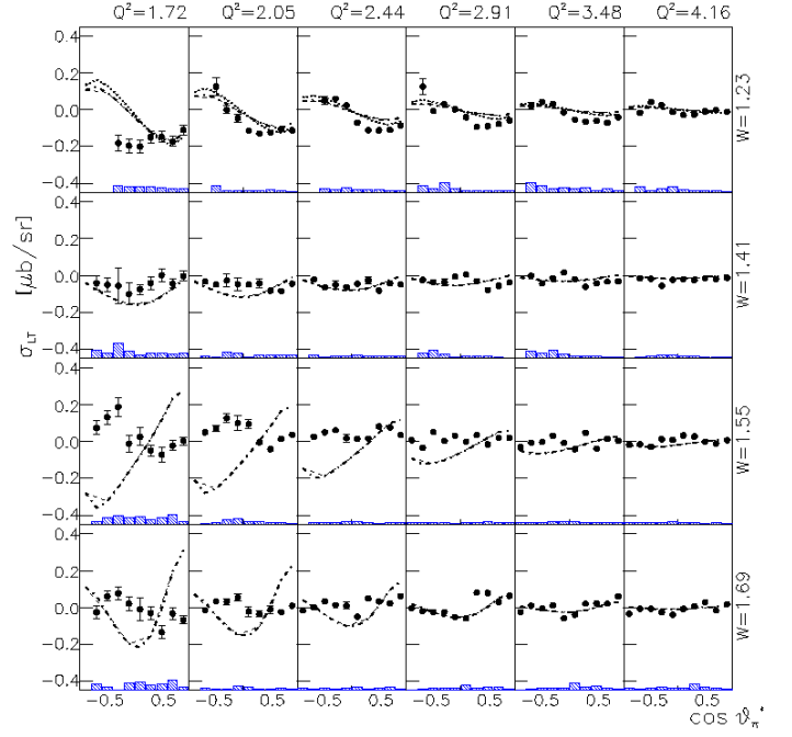
FIG. 18: Structure function \sigma_{LT} as a function of \cos \theta_\pi^* at fixed W and Q^2 compared to model calculations. Curves as in Fig. 15. Systematic uncertainties are shown in shaded bars.
