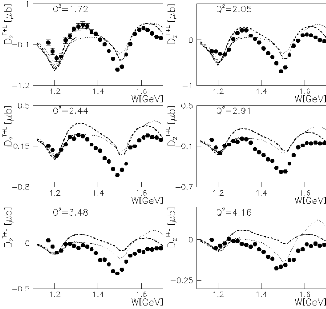
FIG. 23: Legendre moment D_2^{T+L} vs W . Curves as in Fig. 21.
