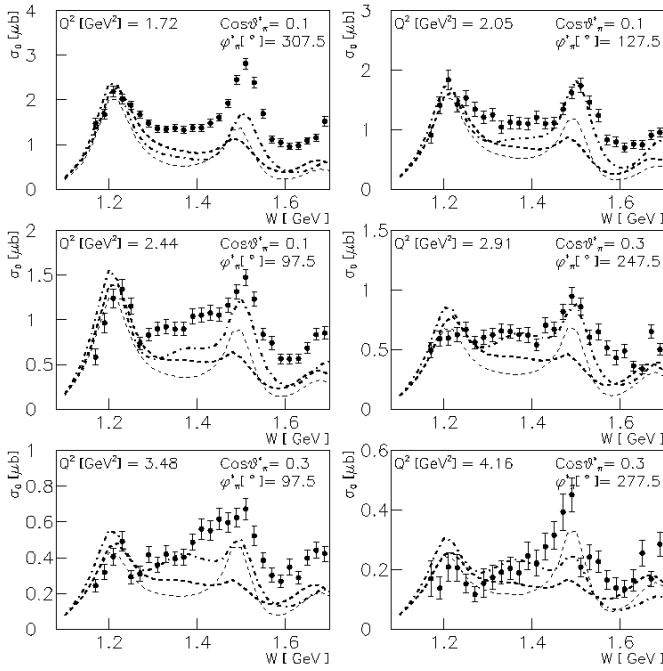
FIG. 13: Samples of differential cross section vs W at different \cos\theta_\pi^* and \phi_\pi^* . Curves as in Fig. 11. \sigma_0 is defined by Eq. 13.
