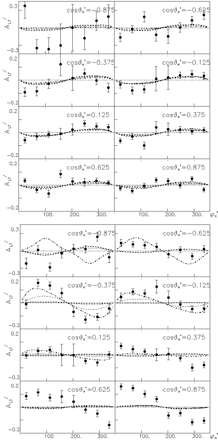
FIG. 14: Electron beam helicity asymmetry as a function \phi_\pi^* in different \cos\theta_\pi^* bins at W = 1.40 GeV (top) and W = 1.69 GeV (bottom), Q^2 = 2.05 GeV 2 compared to different physics models MAID98 (thin solid), MAID00 (thin dash), MAID03 (bold dash-dot), and DMT (bold dash)
