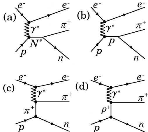
FIG. 2: Tree level description of single \pi^+ electroproduction. (a) s -channel resonance production (b) s -channel nucleon exchange (c) t -channel pion exchange (d) t -channel \rho meson exchange
