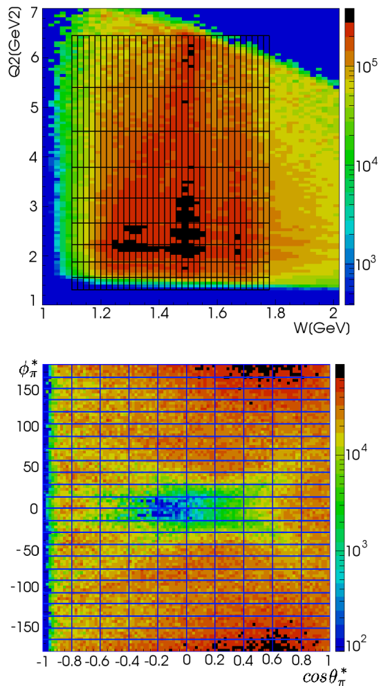
FIG. 9: (Color online) Kinematic coverage in Q^2 [GeV ^2 ] versus W [GeV](top) and in \phi_\pi^* versus \cos\theta_\pi^* (bottom). The solid lines show the bins used in the data analysis.
