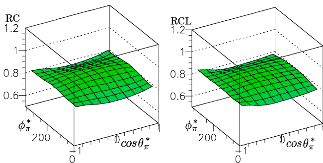
FIG. 10: Examples of ExcluRad results of radiative correction factors for the pion production cross section at a specific kinematics in W = 1.40 GeV, Q^2 = 1.7 GeV 2 . The left graph shows the exact calculation, the right panel shows the leading log approximation.
