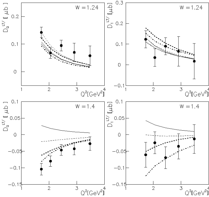
FIG. 20: The Q^2 dependence of Legendre moments of \sigma_{LT'} for \pi^+ channel at W = 1.24, 1.4 GeV. Curves as in Fig. 19.
