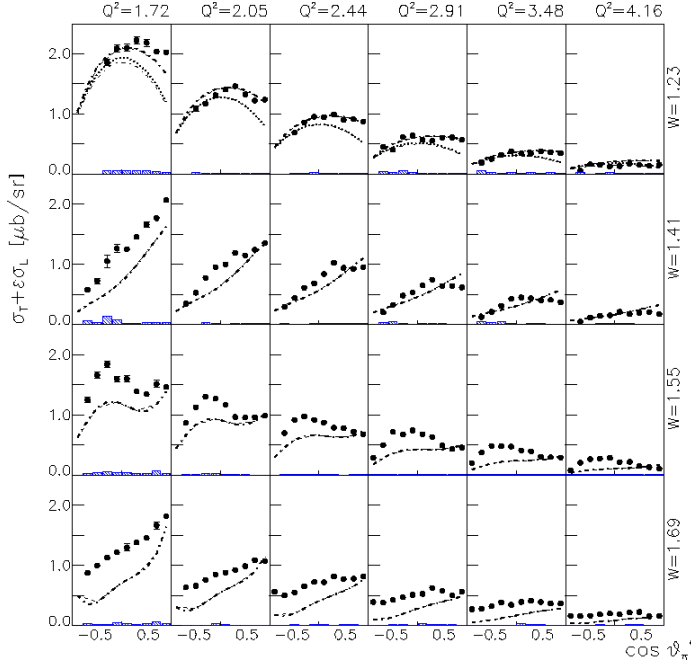
FIG. 15: Structure function \sigma_T + \epsilon\sigma_L as a function of \cos \theta_\pi^* for different W and Q^2 values in comparison with model calculations MAID00(thin dash), MAID03(bold dash-dot), SL(bold dot) and SL04(thin dash-dot). The shaded bars shows the systematic uncertainties.
