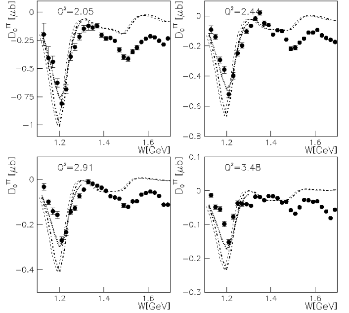
FIG. 25: Legendre moment D_0^{TT} of the structure function \sigma_{TT} vs W . Curves as in Fig. 21.
