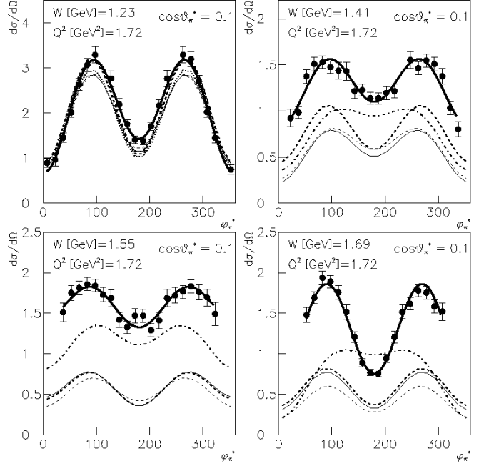
FIG. 12: Examples of differential cross section [ \mu\text{b}/\text{sr} ] at fixed Q^2 , \cos\theta_\pi^* \text{ vs } \phi_\pi^* for different W . DMT (bold dash), MAID98 (thin solid), MAID00 (thin dashed), MAID03 (bold dash-dot), SL (bold dot) and SL04 (thin dash-dot). The bold solid line is the result of the A + B \cos\phi_\pi^* + C \cos 2\phi_\pi^* fit to the data .
