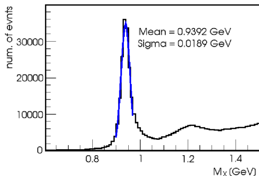
FIG. 7: Missing mass M_X distribution for ep \rightarrow e\pi^+X events.
