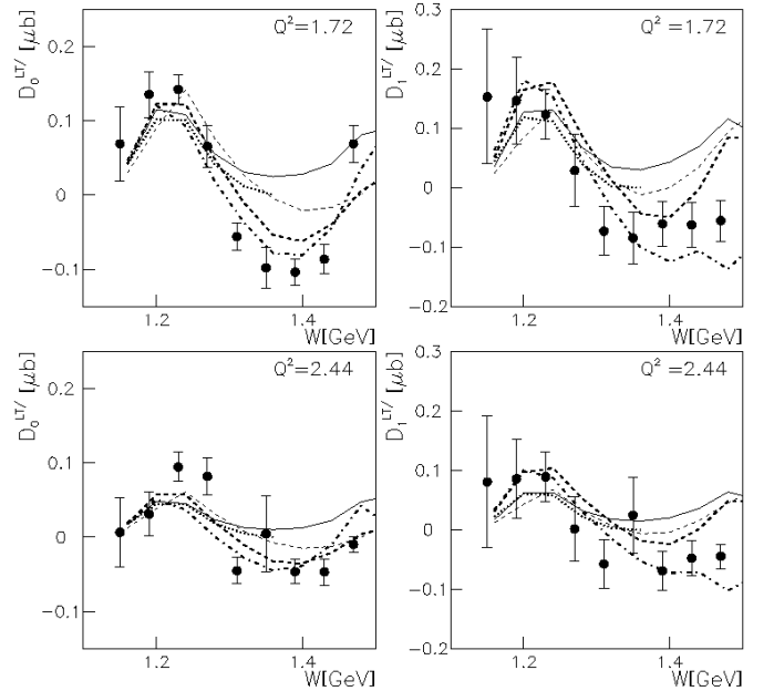
FIG. 19: Legendre moment D_0^{LT'} , D_1^{LT'} of \sigma_{LT'} vs W . Model predictions: MAID98(thin solid), MAID00(thin dash), MAID03(bold dash-dot), SL(bold dot), and DMT(bold dash)
