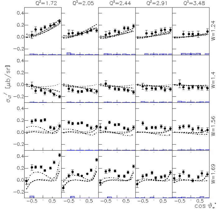
FIG. 16: Structure function \sigma_{LT'} as a function of \cos \theta_\pi^* at fixed W and Q^2 compared to model calculations. Curves as in Fig. 15. Systematic uncertainties are shown in shaded bars.
