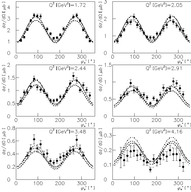
FIG. 11: Differential cross section vs \phi_\pi^* in the \Delta(1232) region at fixed \cos\theta_\pi^* = -0.1 for different bins in Q^2 . DMT (bold dash), MAID00 (thin dash), MAID03 (bold dash-dot) and SL04 (thin dash-dot). The error bar of data shows only statistical error.
