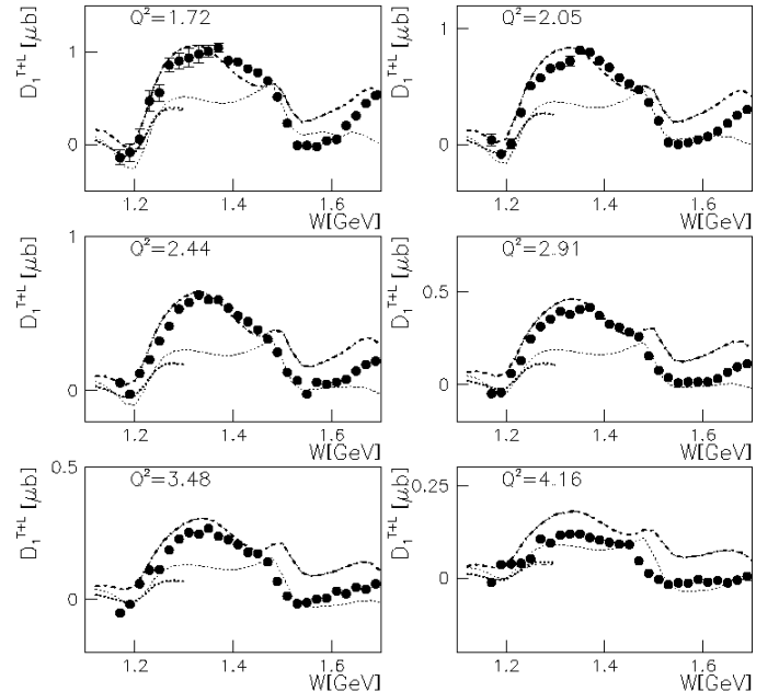
FIG. 22: Legendre moment D_1^{T+L} . Curves as in Fig. 21.
