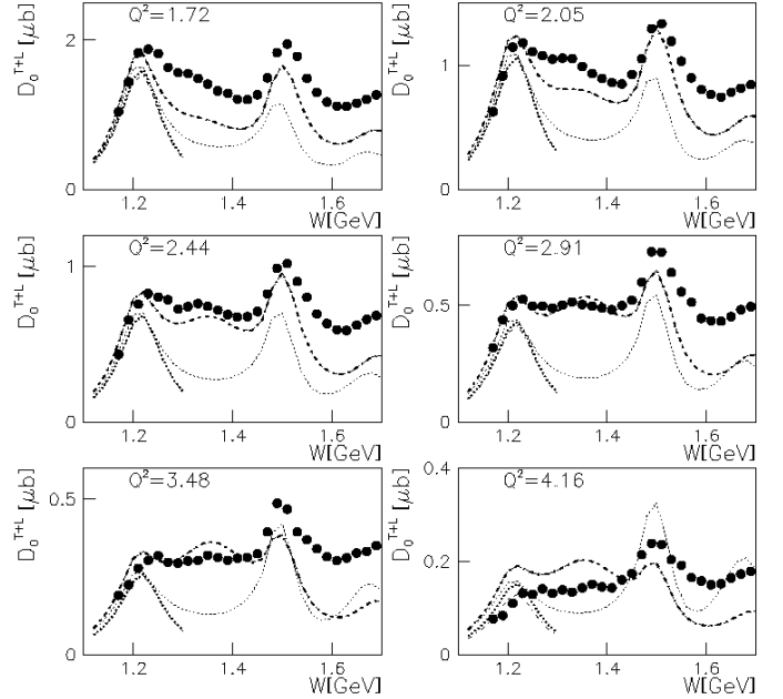
FIG. 21: Legendre moment D_0^{T+L} of structure function \sigma_T + \epsilon\sigma_L vs W . Curves: MAID03(bold dash-dot), MAID00(thin dash), SL(bold dot), SL04(thin dash-dot) and MAID00 with the P_{11}(1440) amplitudes switched off(thin dot).
