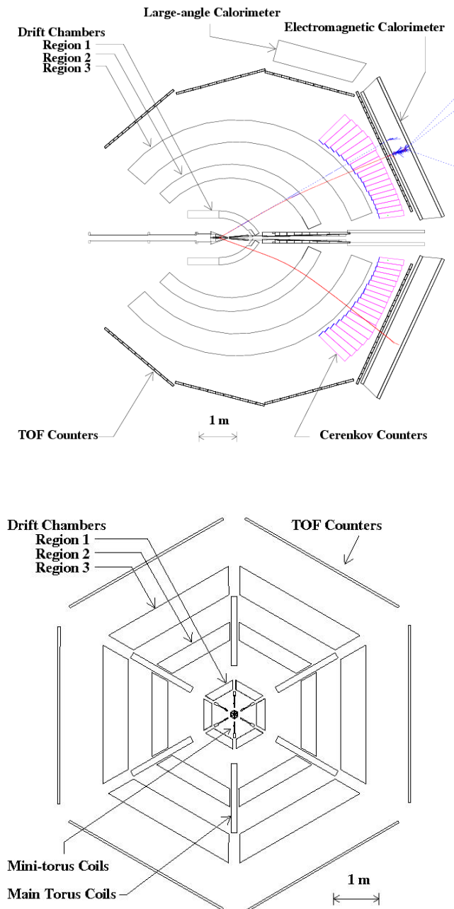
FIG. 3: (Color online) Schematics of the CLAS detector system. The top panel shows a cut through sectors 1 and 4 along the beam line. The beam enters from the left into CLAS. A GEANT-simulated event is shown with an electron bending towards the beam line and a positive particle in the opposite sector bending away from the beam. The bottom panel shows a cut perpendicular to the beam line through the center of CLAS.
