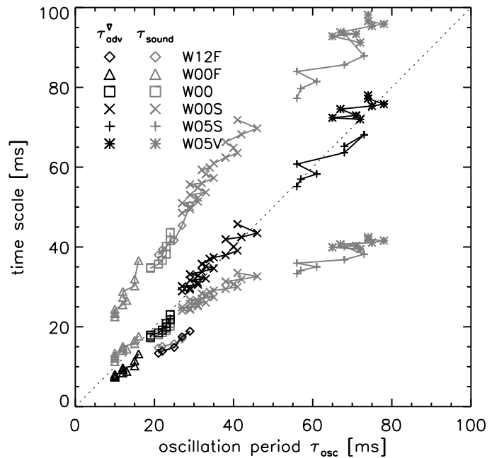
Fig. 16. Advection time \tau_{\text{adv}}^{\nabla} of the fluid moving from the shock to the radius of maximum deceleration, R_{\nabla} , and the two acoustic times \tau_{\text{sound}}^{\text{rad}} (lower grey symbols) and \tau_{\text{sound}}^{\text{lat}} (upper grey symbols), versus the oscillation period, \tau_{\text{osc}} , for Models W00F, W00, W00S, W05S, W05V and W12F. The data used in this figure are selected from phases in which the oscillations can be clearly identified and in which the flow is quasi-stationary (see Fig. 15). While \tau_{\text{sound}}^{\text{lat}} is clearly too long in all cases and \tau_{\text{sound}}^{\text{rad}} is too short for all models except W00 and W00F, the oscillation period is well approximated by \tau_{\text{adv}}^{\nabla} for all models except W12F. The special role of Model W12F can be explained by the effects of strong neutrino heating (see text).
