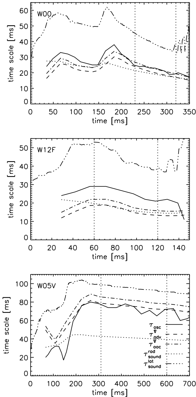
Fig. 15. Evolution of the l = 1 mode oscillation period, \tau_{\text{osc}} , the advection time \tau_{\text{adv}}^{\nabla} from the shock to the radius R_{\nabla} of strongest deceleration, and the time \tau_{\text{aac}}^{\nabla} for a radial advective-acoustic cycle, for Models W00, W12F and W05V. The advection time \tau_{\text{adv}}^{\nabla} agrees with the oscillation time for Models W00 and W05V. In Model W12F, the oscillation period is longer than both \tau_{\text{adv}}^{\nabla} and \tau_{\text{aac}}^{\nabla} , which can be explained by the consequences of strong neutrino heating (see text). The oscillation period is also compared to the radial sound travel time \tau_{\text{sound}}^{\text{rad}} through the shock cavity and back, and the maximum lateral sound travel time \tau_{\text{sound}}^{\text{lat}} just behind the shock. \tau_{\text{osc}} is close to \tau_{\text{sound}}^{\text{rad}} for Model W00, but is closer to \tau_{\text{sound}}^{\text{lat}} for Model W05V. The vertical dotted lines enclose the time intervals considered for the evaluations of Figs. 16 and 17.
