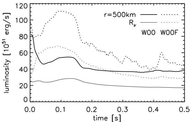
Fig. 18. Evolution of the sum of the \nu_e and \bar{\nu}_e luminosities at the neutrinosphere and at r = 500 \text{ km} for Models W00 and W00F. The luminosities decay with time because the largest mass accretion rates are present at early times ( t < 0.2 \text{ s} ). Model W00F has the higher luminosity, because the neutron star contracts faster, setting free more gravitational energy.
