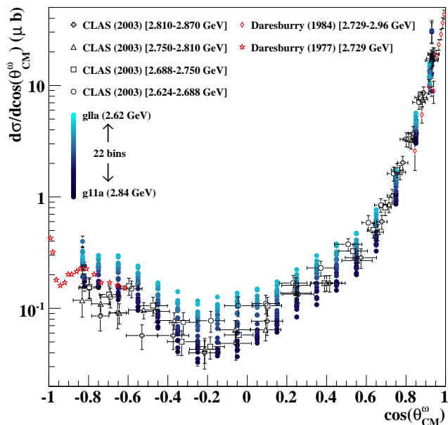
FIG. 11: (Color Online) \frac{d\sigma}{d\cos\theta_{CM}^\omega} (\mu\text{b}) vs. \cos\theta_{CM}^\omega : Comparison of the present CLAS results (blue circles) with previously published results from CLAS [4] (black open crosses, triangles, squares and circles) and Daresbury [2, 3] (red open diamonds and stars) in the energy range 2.62 \text{ GeV} < W < 2.96 \text{ GeV} . The Daresbury (1977) points have no error bars; the points were extracted from a portable document format (PDF) image.
