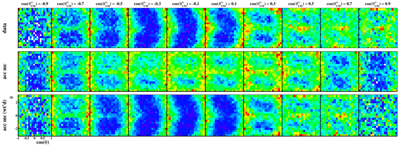
FIG. 6: (Color Online) \phi vs. \cos\theta in the Adair frame (see Section VIII B) in \cos\theta_{CM}^\omega bins: Example fit result in the W = 2.005 GeV bin for data (top row), phase space accepted Monte Carlo events (middle row) and phase space accepted Monte Carlo events weighted by the fits discussed in Section V (bottom row). Note that the weighted Monte Carlo provides an accurate description of the data ( \chi^2/\text{degrees-of-freedom} \sim 0.6 ).
