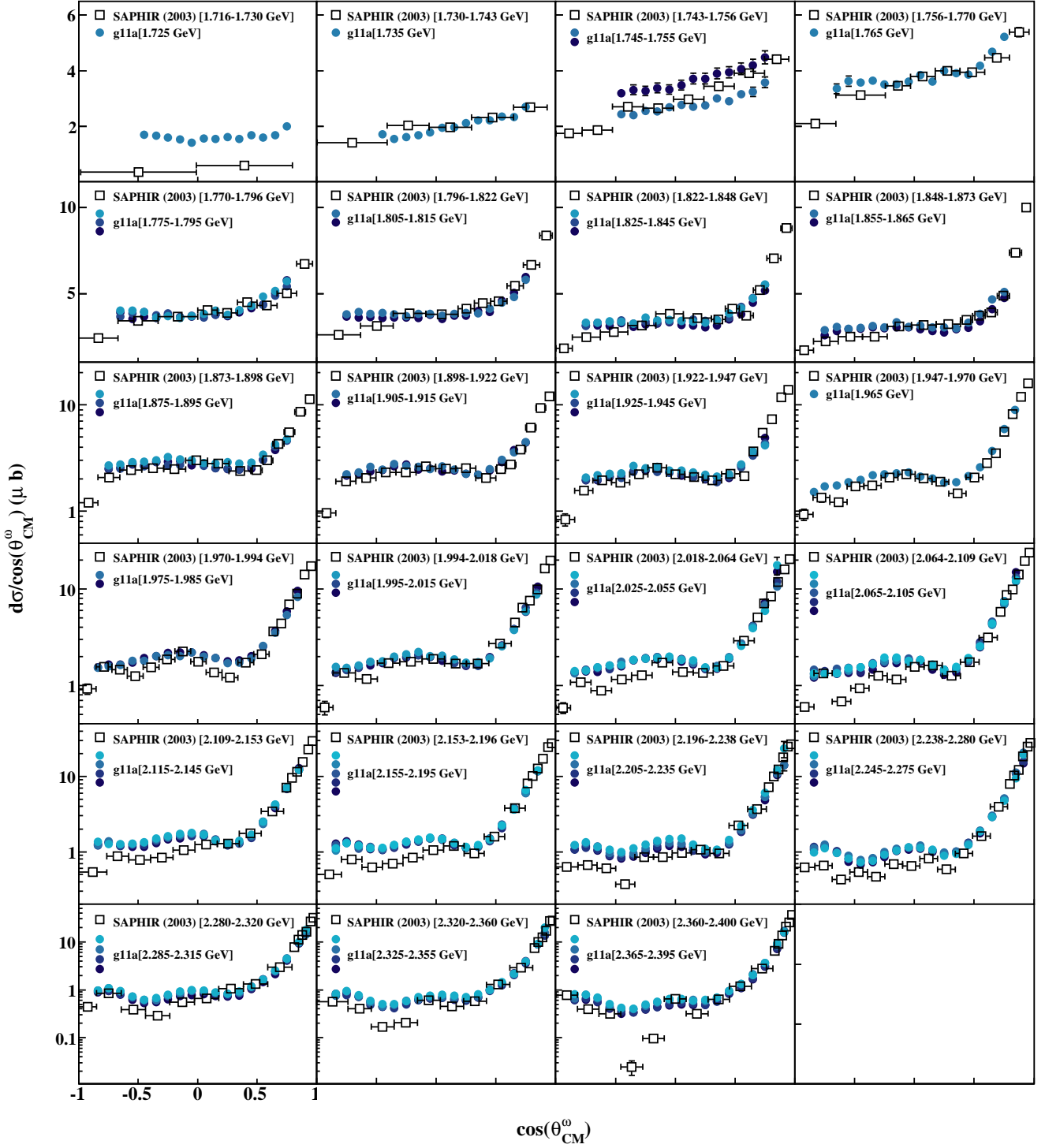
FIG. 12: (Color Online) \frac{d\sigma}{d\cos\theta_{CM}^0}(\mu b) vs. \cos\theta_{CM}^0 : Comparison of the present CLAS results (blue circles) with previously published results from SAPHIR [5] (black open squares).
