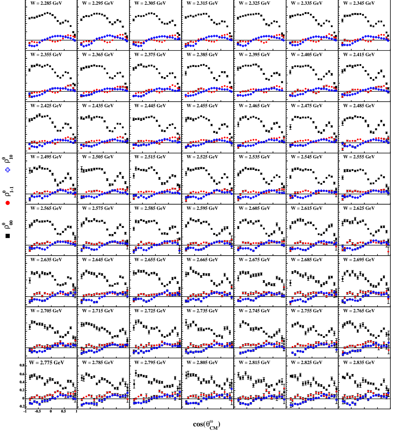
FIG. 10: (Color Online) \rho_{MM'}^0 vs. \cos\theta_{CM}^{\omega} : Spin density matrix element measurements, in the Adair frame, for bins in the range 2.28 \text{ GeV} \leq W < 2.84 \text{ GeV} . The black squares are \rho_{00}^0 , the red circles are \rho_{1-1}^0 and the blue crosses are \text{Re}(\rho_{10}^0) . The centroid of each 10-MeV wide bin is printed on the plot. The error bars do not include systematic uncertainties.
