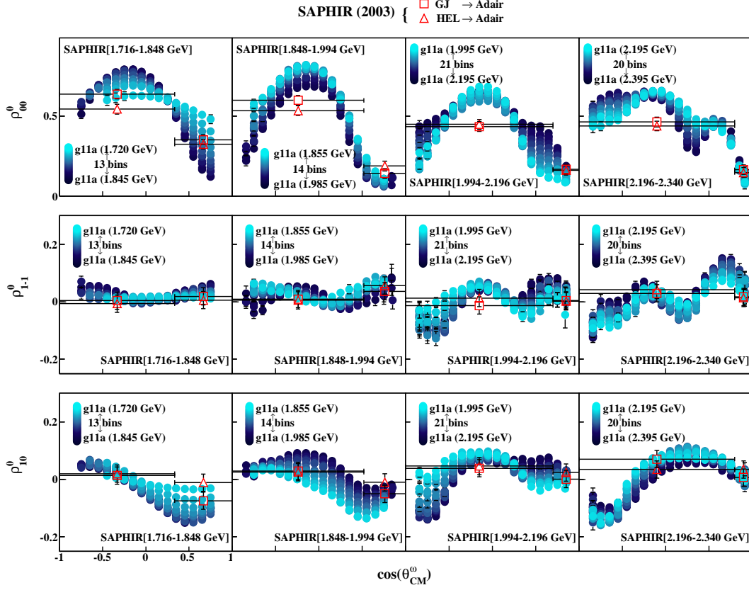
FIG. 13: (Color Online) \rho_{MM'}^0 in the Adair frame vs. \cos\theta_{CM}^\omega : Comparison of the present CLAS results (blue circles) with previously published SAPHIR [5] results (open red squares and triangles). SAPHIR extracted results independently in the Gottfried-Jackson and Helicity frames — both presented here rotated to the Adair frame.
