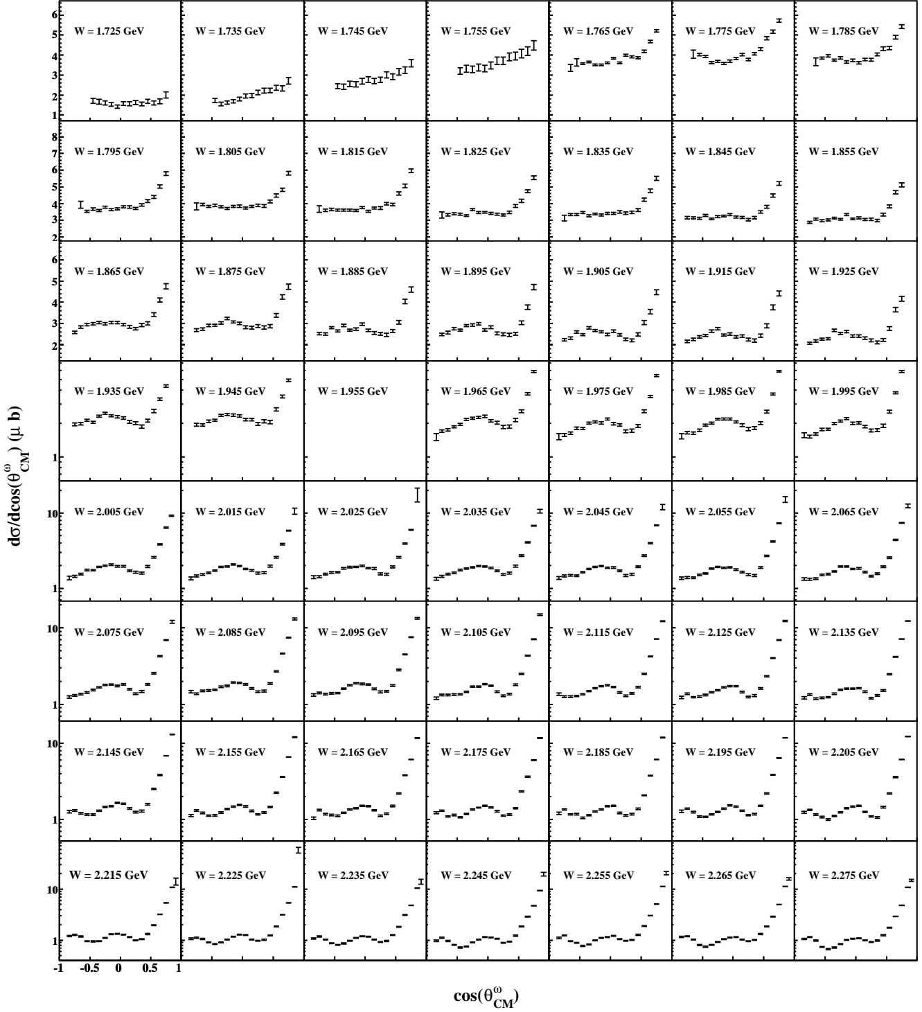
FIG. 7: \frac{d\sigma}{d\cos(\theta_{CM}^\omega)} ( \mu\text{b} ) vs. \cos(\theta_{CM}^\omega) : Differential cross section results for bins in the energy range 1.72 \text{ GeV} \leq W < 2.28 \text{ GeV} . The centroid of each 10-MeV wide bin is printed on the plot. The lack of reported data points in the W = 1.955 GeV bin is discussed in Section VI. The error bars, which do not include systematic uncertainties, are discussed in the text. The additional near-threshold background separation uncertainties, discussed in Section IV, are clearly visible in the first four center-of-mass energy bins. Note that the vertical scales are linear below W of 1.935 GeV and linear above that.
