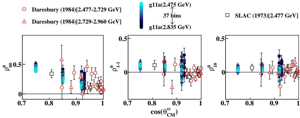
FIG. 14: (Color Online) \rho_{MM'}^0 in the Adair frame vs. \cos\theta_{CM}^\omega : Comparison of the present CLAS results (blue circles) with previously published Daresbury [3] (open red circles and triangles) and SLAC [1] (open black squares).
