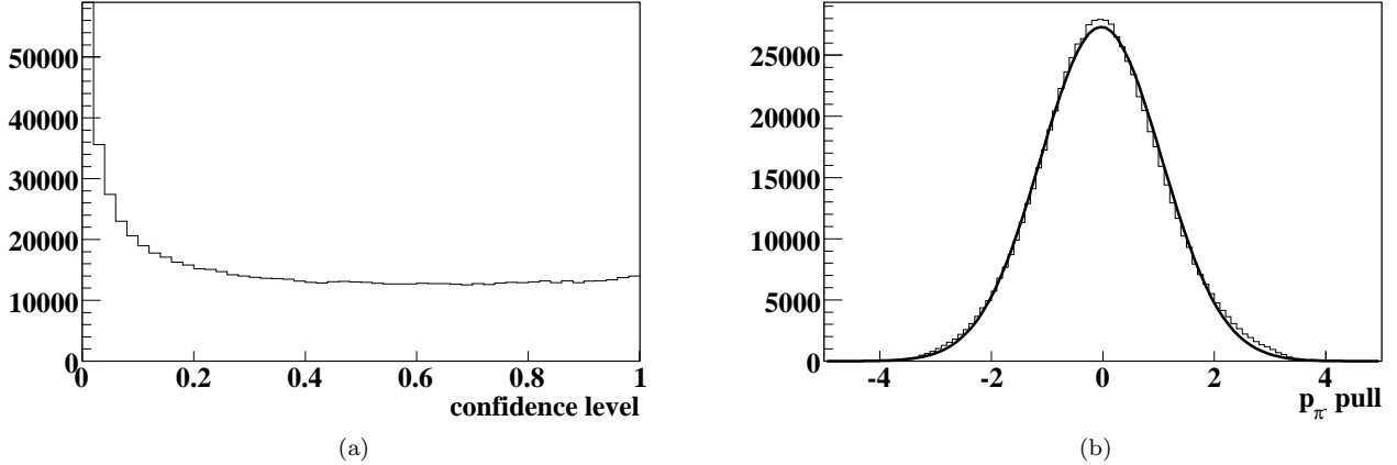
FIG. 1: (a) The confidence levels resulting from 4-constraint kinematic fits performed on a sample of events to the hypothesis \gamma p \rightarrow p\pi^+\pi^- integrated over all kinematics. The “peak” near zero consists of events that do not match the hypothesis, along with poorly measured (due to multiple scattering, etc. ) signal events. Agreement with the ideal (flat) distribution for signal events is very good. (b) Example pull-distribution for the momentum of the \pi^- from the same kinematic fits as in (a). Only events with a confidence level larger than 1% are shown. The line represents a Gaussian fit to this distribution. For this event sample, the parameters obtained are \mu = -0.029 \pm 0.001 , \sigma = 1.086 \pm 0.001 (the uncertainties are purely statistical), which are in very good agreement with the ideal values \mu = 0, \sigma = 1 . Both (a) and (b) are good indicators that the CLAS error matrix is well understood.
