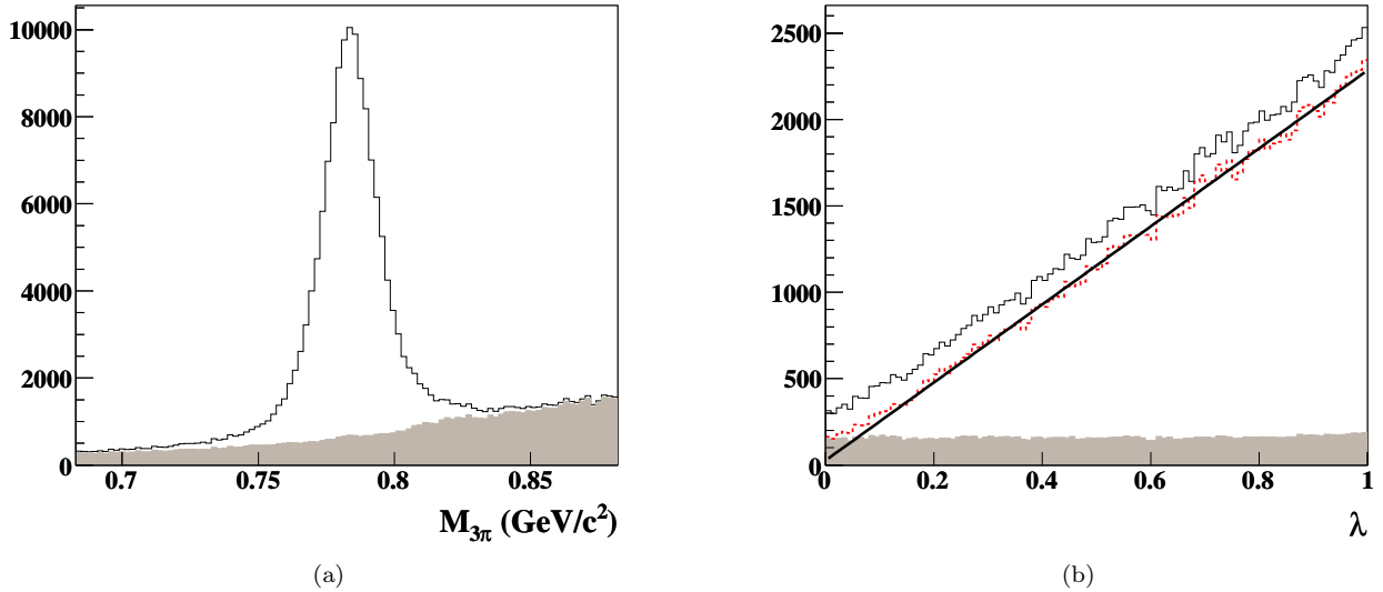
FIG. 3: (Color Online) (a) The 3\pi invariant mass distribution in the W = 2.205 GeV bin, integrated over all kinematics, for all events (unshaded) and for events weighted by the background factors, 1 - Q (shaded). (b) The \lambda distribution of events in the same W bin that satisfy |M_{3\pi} - M_\omega| < 25 MeV/ c^2 (unshaded), the same events weighted by signal factors Q (dashed-red), and by background factors 1 - Q (shaded). The line represents a fit of the signal to the function a\lambda .
