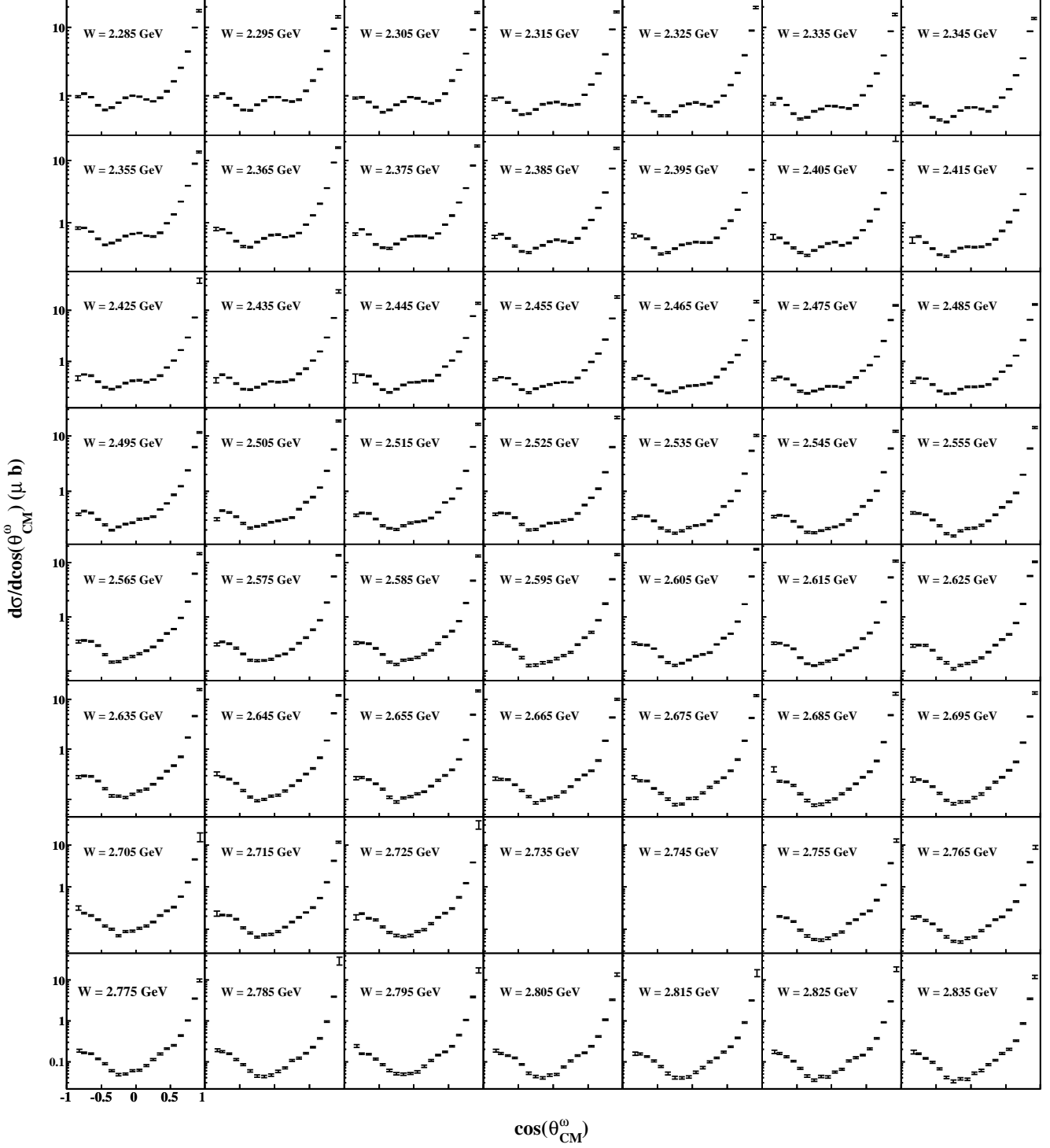
FIG. 8: \frac{d\sigma}{d\cos\theta_{CM}^\omega} ( \mu\text{b} ) vs. \cos\theta_{CM}^\omega : Differential cross section results for bins in the energy range 2.28 \text{ GeV} \leq W < 2.84 \text{ GeV} . The centroid of each 10-MeV wide bin is printed on the plot. The lack of reported data points in the W = 2.735 \text{ GeV} and W = 2.745 \text{ GeV} bins is discussed in Section VI. The error bars, which do not include systematic uncertainties, are discussed in the text.
