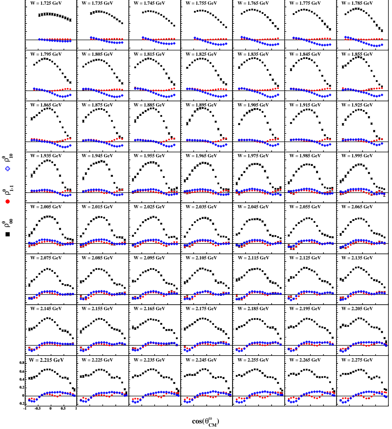
FIG. 9: (Color Online) \rho_{MM}^0 vs. \cos\theta_{CM}^{\omega} : Spin density matrix element measurements, in the Adair frame, for bins in the range 1.72 \text{ GeV} \leq W < 2.28 \text{ GeV} . The black squares are \rho_{00}^0 , the red circles are \rho_{1-1}^0 and the blue crosses are Re(\rho_{10}^0) . The centroid of each 10-MeV wide bin is printed on the plot. The error bars do not include systematic uncertainties.
