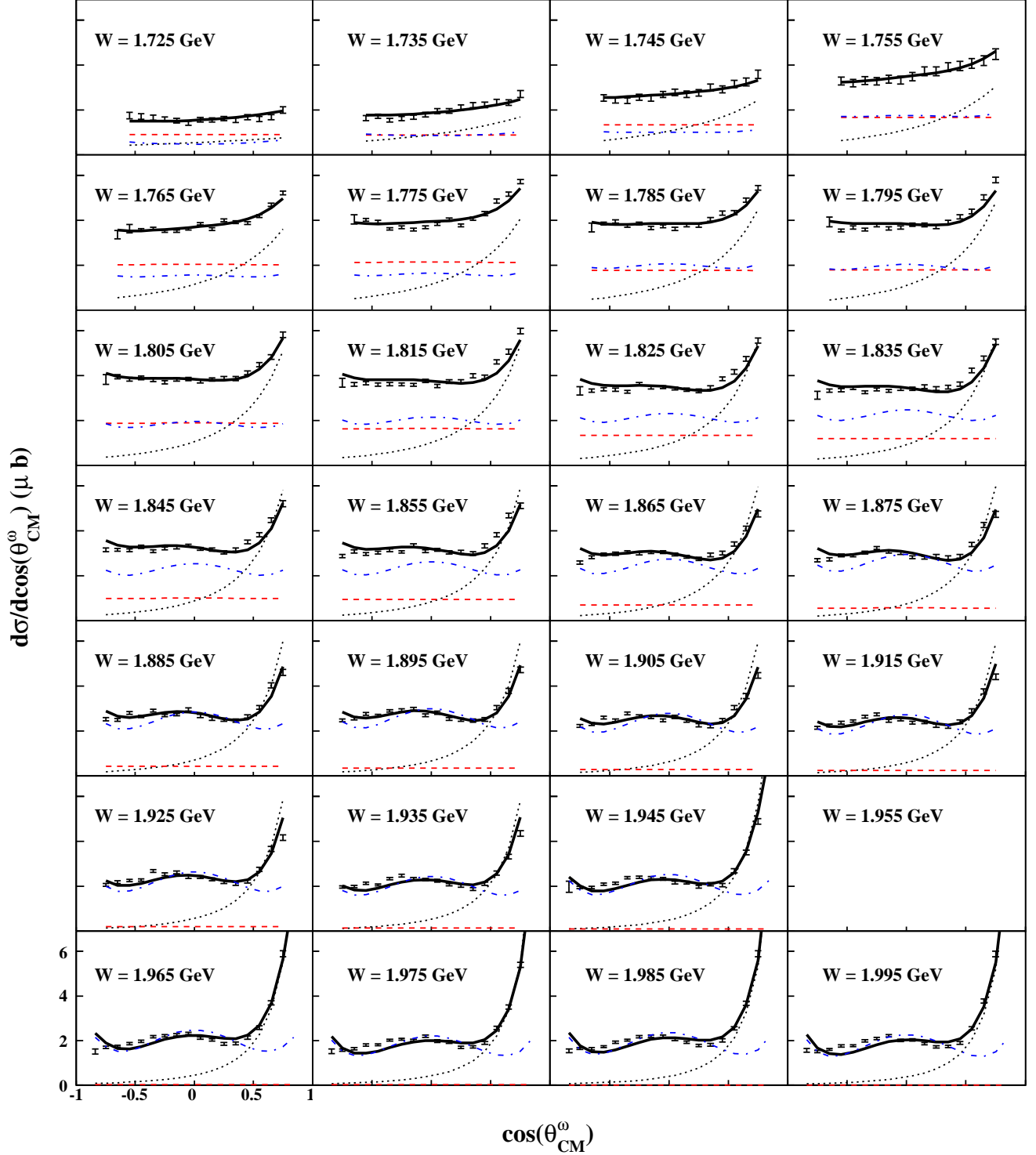
FIG. 5: (Color Online) d\sigma/d\cos\theta_{CM}^\omega(\mu\text{b}) vs \cos\theta_{CM}^\omega : PWA results from Fit I (solid black line), compared to our measurements [11]. The individual contributions from the J^P = 3/2^- wave (dashed red line), J^P = 5/2^+ wave (dashed-dotted blue line) and OTL t -channel terms (dotted black line) are also shown. The lack of data reported in the W = 1.955 GeV bin is due to normalization issues [11].
