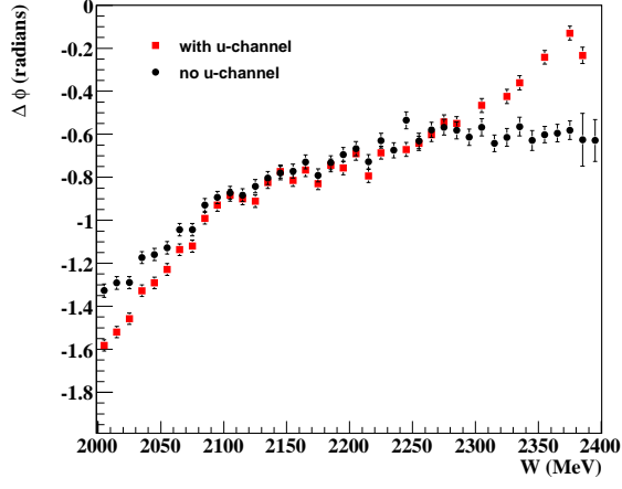
FIG. 14: Fit II + u -channel: \Delta\phi = \phi_{7/2-} - \phi_{5/2+} (radians) vs W(\text{MeV}) : Phase motion obtained with and without u -channel terms in Fit II. Including u -channel terms only creates discrepancies in the phase motion where one of the s -channel waves has a small contribution to the cross section. The error bars on both phase motion plots are purely statistical.
