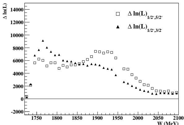
FIG. 2: \Delta \ln \mathcal{L} vs W(\text{MeV}) : Example likelihood differences from s -channel scans. Each fit contained the locked OTL t -channel terms, along with a single s -channel wave. Shown are \Delta \ln \mathcal{L}_{1/2^+, 5/2^+} = \ln \mathcal{L}_{5/2^+} - \ln \mathcal{L}_{1/2^+} (open squares) and \Delta \ln \mathcal{L}_{1/2^+, 3/2^-} = \ln \mathcal{L}_{3/2^-} - \ln \mathcal{L}_{1/2^+} (closed triangles). See text for details and discussion.
