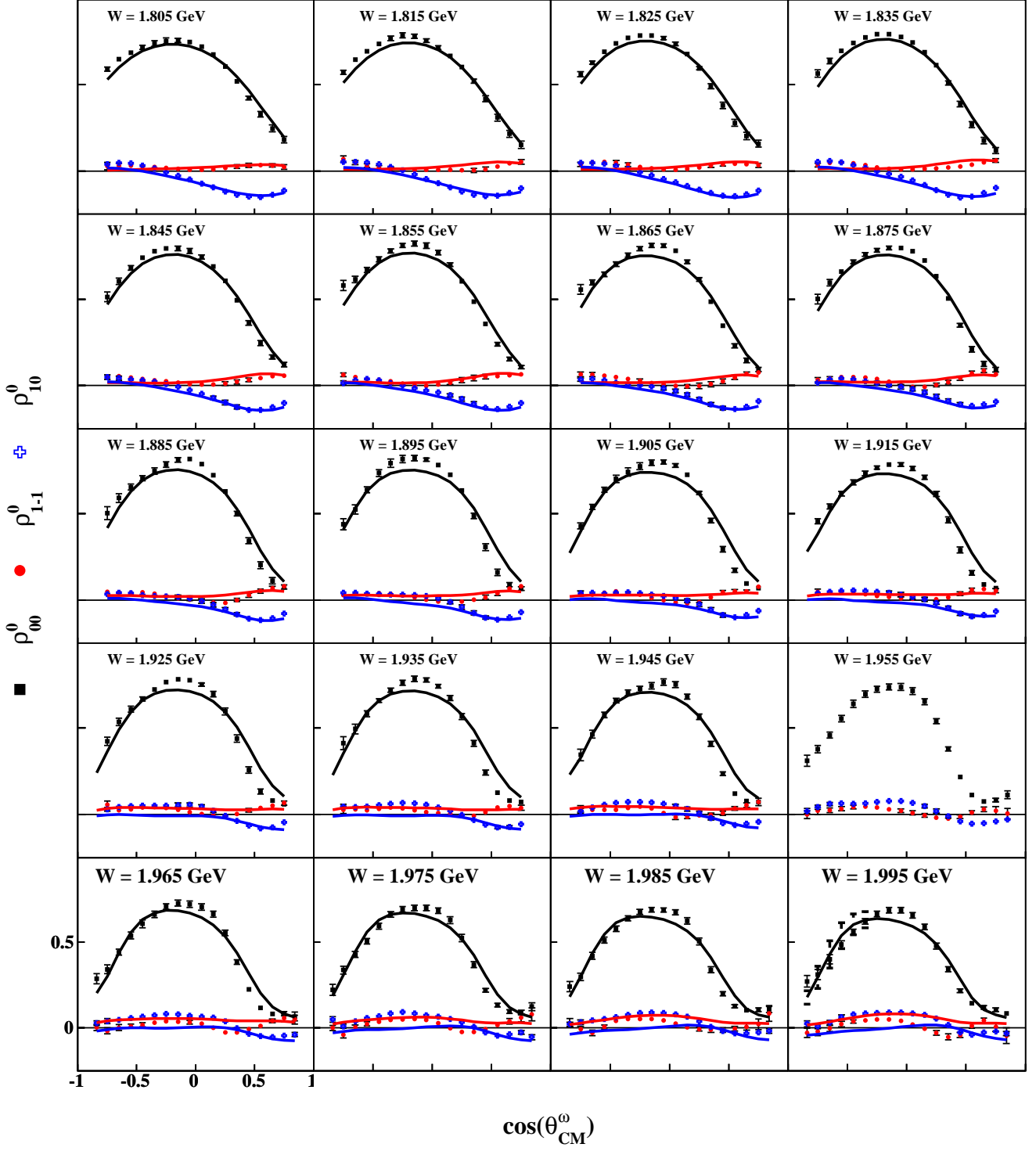
FIG. 13: (Color Online) \rho_{MM'}^0 vs \cos\theta_{CM}^{\omega} : PWA results from Fit III: \rho_{00}^0 (solid black line), \rho_{1-1}^0 (solid red line), Re\rho_{10}^0 (solid blue line), compared to our measurements [11]. No fit was performed in the W = 1.955 GeV bin, see text for details.
