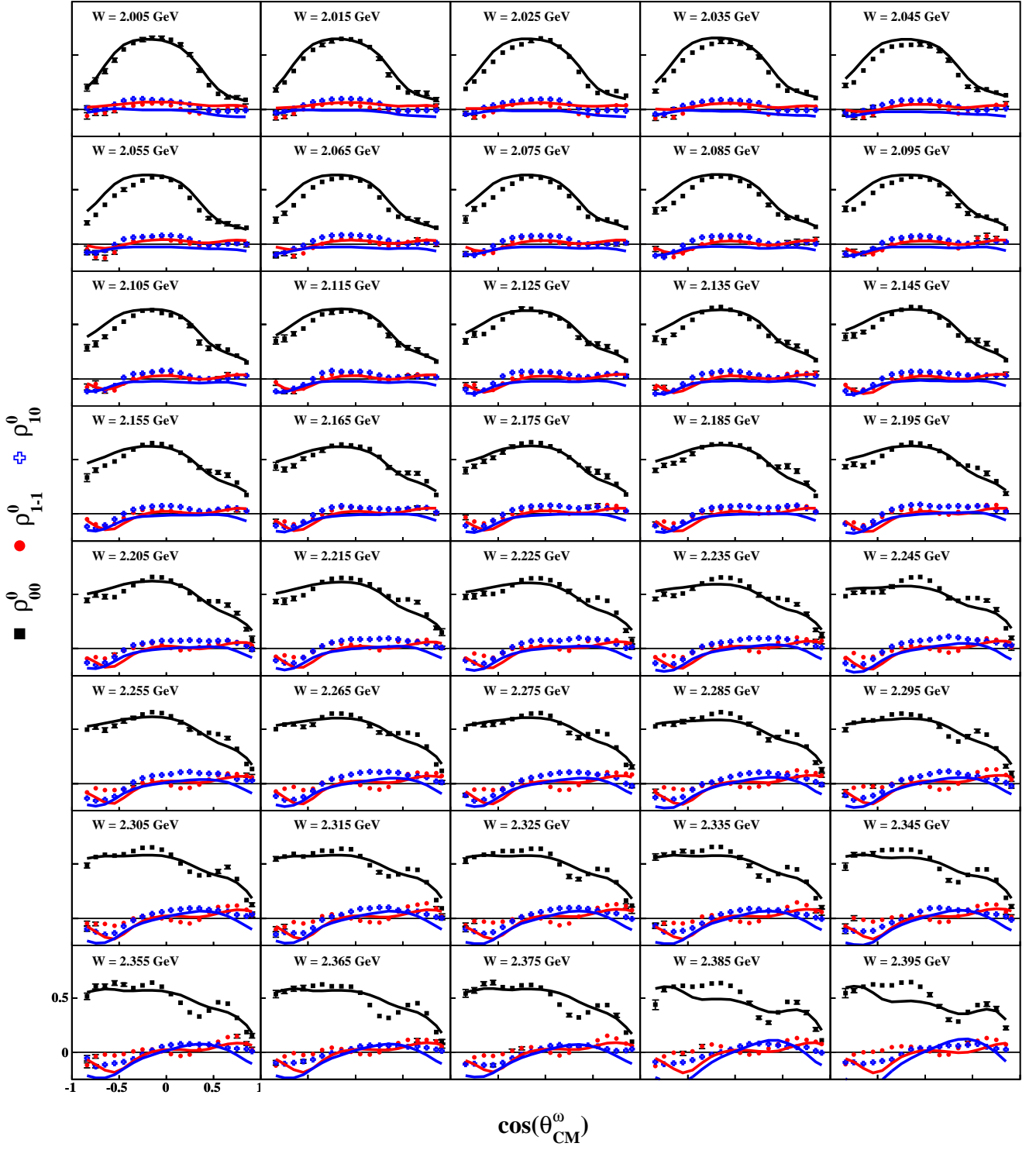
FIG. 10: (Color Online) \rho_{MM'}^0 vs \cos\theta_{CM}^0 : PWA results from Fit II: \rho_{00}^0 (solid black line), \rho_{1-1}^0 (solid red line), Re\rho_{10}^0 (solid blue line), compared to our measurements [11]. See text for discussion.
