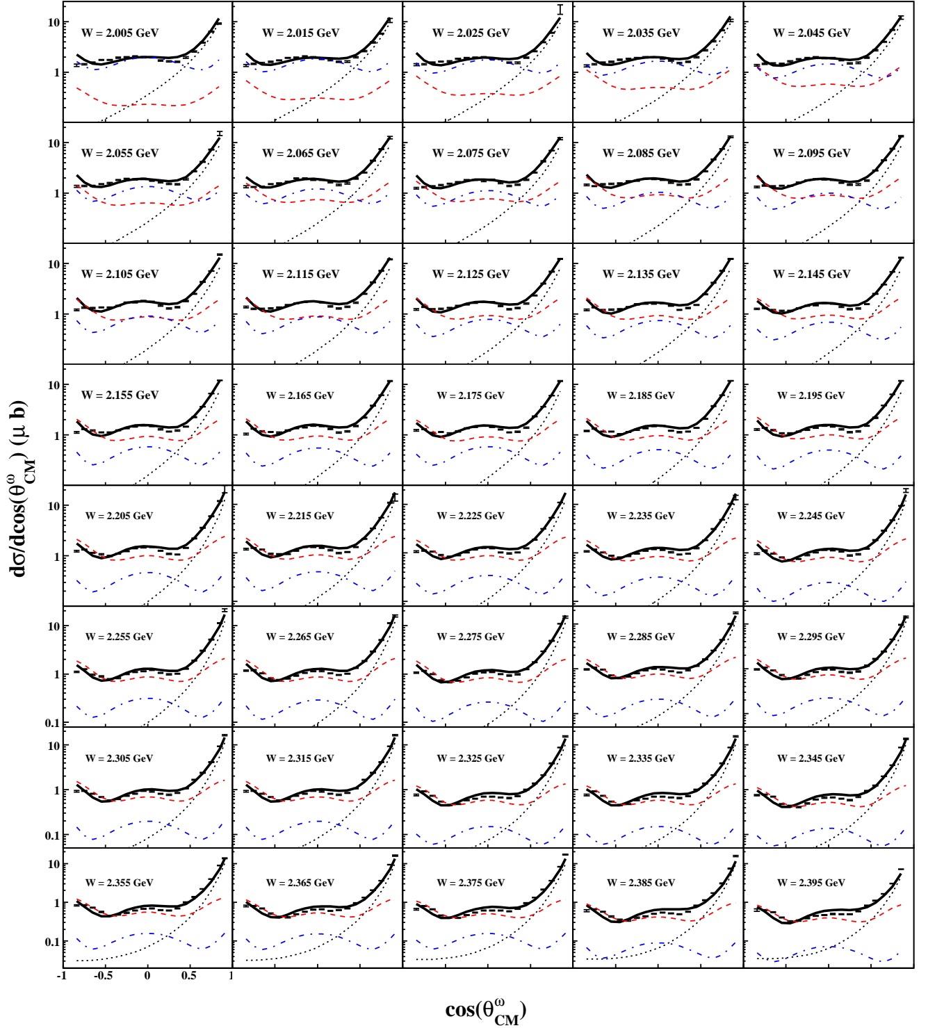
FIG. 9: (Color Online) d\sigma/d\cos\theta_{CM}^0(\mu b) vs \cos\theta_{CM}^0 : PWA results from Fit II (solid black line), compared to our measurements [11]. The individual contributions from the J^P = 7/2^- wave (dashed red line), J^P = 5/2^+ wave (dashed-dotted blue line) and OTL t -channel terms (dotted black line) are also shown.
