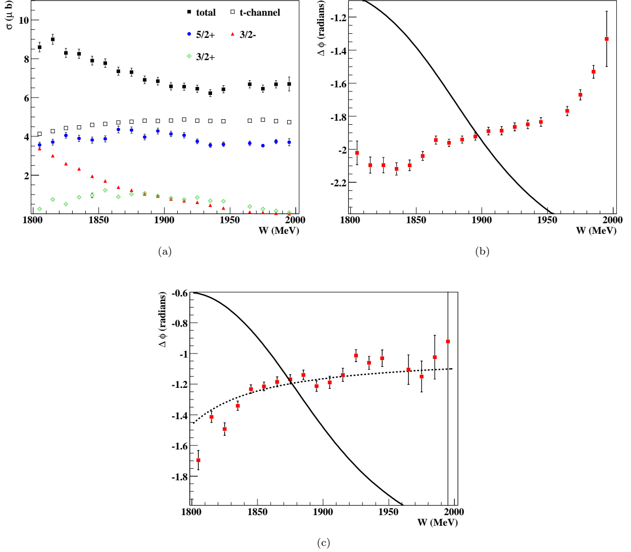
FIG. 11: Results from Fit III: (a) \sigma(\mu\text{b}) vs W(\text{MeV}) : Total cross sections extracted from all of the waves in the fit (filled black squares), only t -channel waves (open squares), only 5/2^+ waves (circles), only 3/2^- waves (triangles) and only 3/2^+ waves (crosses). (b) \Delta\phi = \phi_{5/2^+} - \phi_{3/2^+} (radians) vs W(\text{MeV}) . (c) \Delta\phi = \phi_{3/2^-} - \phi_{3/2^+} (radians) vs W(\text{MeV}) . The solid curves show the phase motion expected assuming the J^P = 3/2^+ has Breit-Wigner parameters M_{3/2^+} = 1875 MeV and \Gamma_{3/2^+} = 150 MeV while locking the J^P = 3/2^- and J^P = 5/2^+ parameters to be those of the D_{13}(1700) and F_{15}(1680) , respectively. The phase motion obtained for the 3/2^+ is not consistent with a single resonant state. The dashed line on (c) represents using the D_{13}(1700) Breit-Wigner parameters for the 3/2^- and a single channel two-pole K-matrix for the 3/2^+ . There is enough freedom to describe the data (see text for discussion). All error bars are purely statistical.
