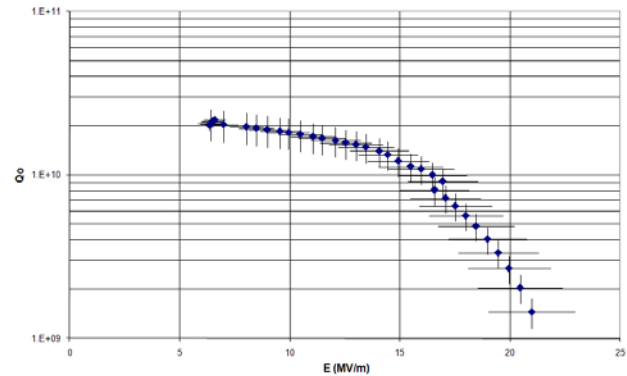
Fig.5: Excitation curve of the cavity treated by the elliptical shape cathode.
