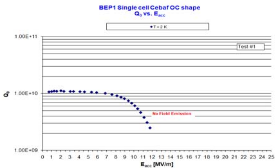
Fig.11: Typical RF test data on CEBAF cavity treated by BEP vertically at JLab employing commercially mixed electrolyte.
