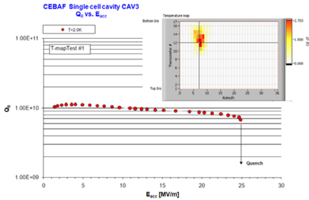
Fig.7: Second RF test result of the cavity treated by the ball shape cathode with thermometry mapping. The insert shows the quench site (please read the text for details).
