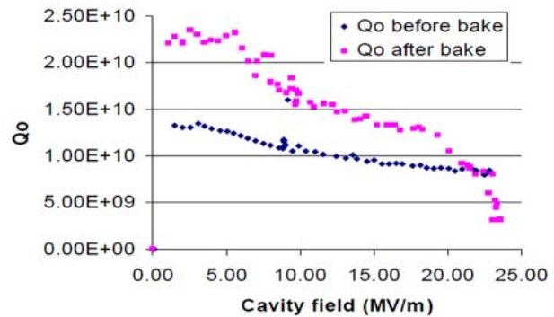
Fig.12: Typical RF test data before and after baking on CEBAF cavity treated by BEP vertically at JLab.
