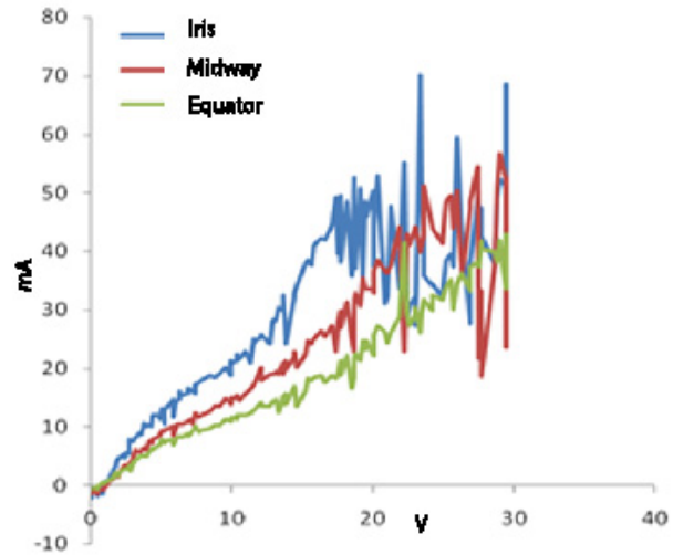
Fig.2: I-V curves of the buttons of the demountable cavity when a pure Al bar was used as the cathode [14]. cathode shape can be important during BEP treatments of Nb SRF single cell cavities. In fact, it was postulated in reference 13 that the cathode shape is important in general for EP of Nb. It was suggested [13] that Nb removal rate could be more homogenous if a shaped cathode that could produce more uniform electric field distribution was used in EP treatments of Nb SRF cavities.
