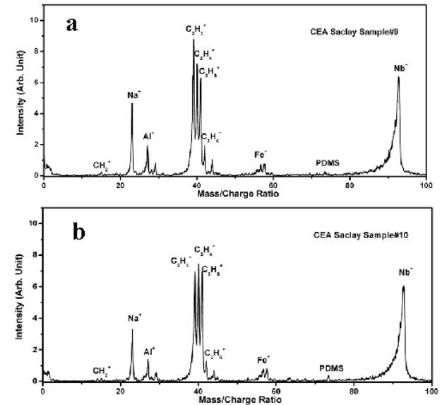
Fig.9: Dynamic SIMS measurements on CEA Saclay's sample#9 a) and sample#10 b). Sample#9 was treated by EP for an Nb removal of 150 \mu\text{m} followed by HF(48%) rinse. Sample#10 was treated by BEP with commercially mixed electrolyte for an Nb removal of 140 \mu\text{m} .
