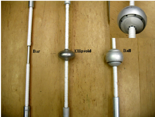
Fig.3: Three different shaped cathodes used in this study. The insert shows bottom view of the ball shape cathode.
