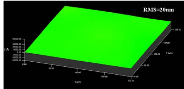
Fig.8: Profilometer image of an Nb sample prepared by PKU's fast BEP technique (please read reference 14).
