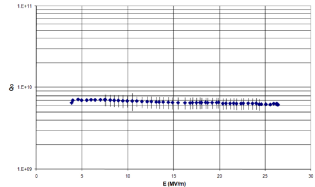
Fig.6: Excitation curve of the cavity treated by the ball shape cathode.
