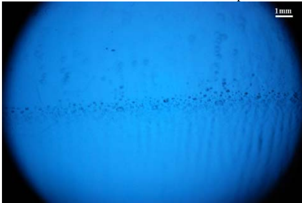
Fig.4: CCD image of the ring of pits located in the midway between iris and equator for the BEP treated Nb single cell cavity via the ball shape cathode (please read the text for details).
