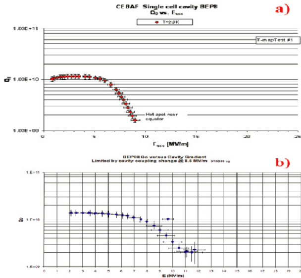
Fig.10: Typical RF test data on CEBAF cavity treated by BEP horizontally at CEA Saclay employing commercially mixed electrolyte: a) after the treated and cleaning, b) after BCP rinsed for two minutes and cleaning.
