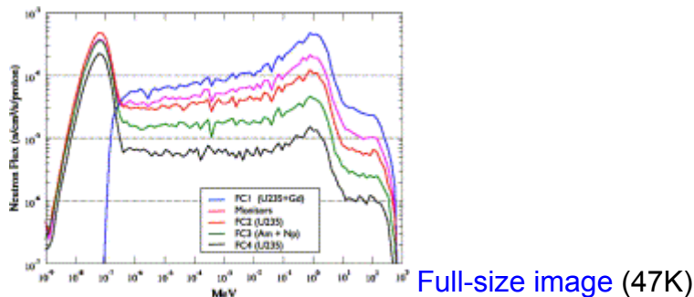
Fig. 2. Simulated neutron fluxes as “seen” by fission chambers (FC), along the beam axis. Minor actinide chambers are not discussed in this paper.
