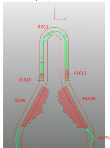
Figure 6: T1 vane profile. Measured profile compared to tolerance (deviation values in mm).
