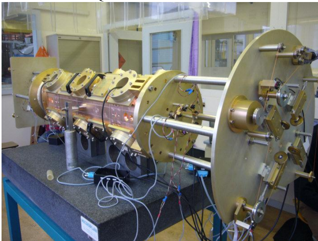
Figure 8: The RFQ RF test bench.
