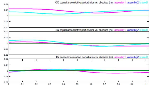
Figure 9: Quadrupole (QQ) and dipole mode capacitance relative errors, measured before (purple) and after (blue) brazing.
