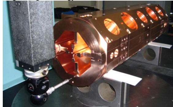
Figure 5: T1 at the CERN metrology workshop after the first brazing.
