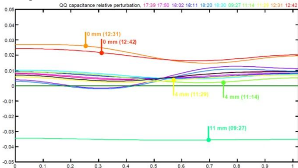
Figure 4: Estimate of the C_{QQ} capacitance error, associated to the fundamental accelerating mode, with vacuum ports at different penetration values (processed data from bead-pull measurements).
