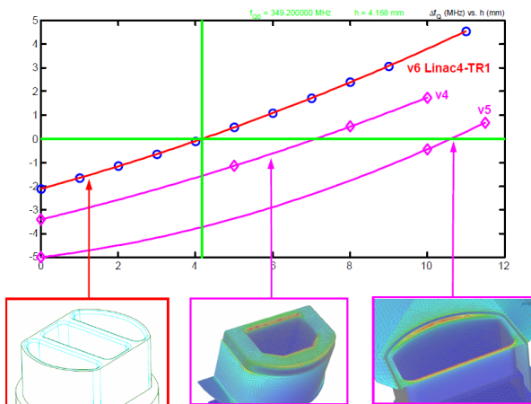
Figure 3: Plot showing the penetration depth for different vacuum port geometries.
