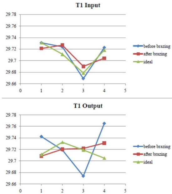
Figure 7: T1 metrology results before and after brazing.
