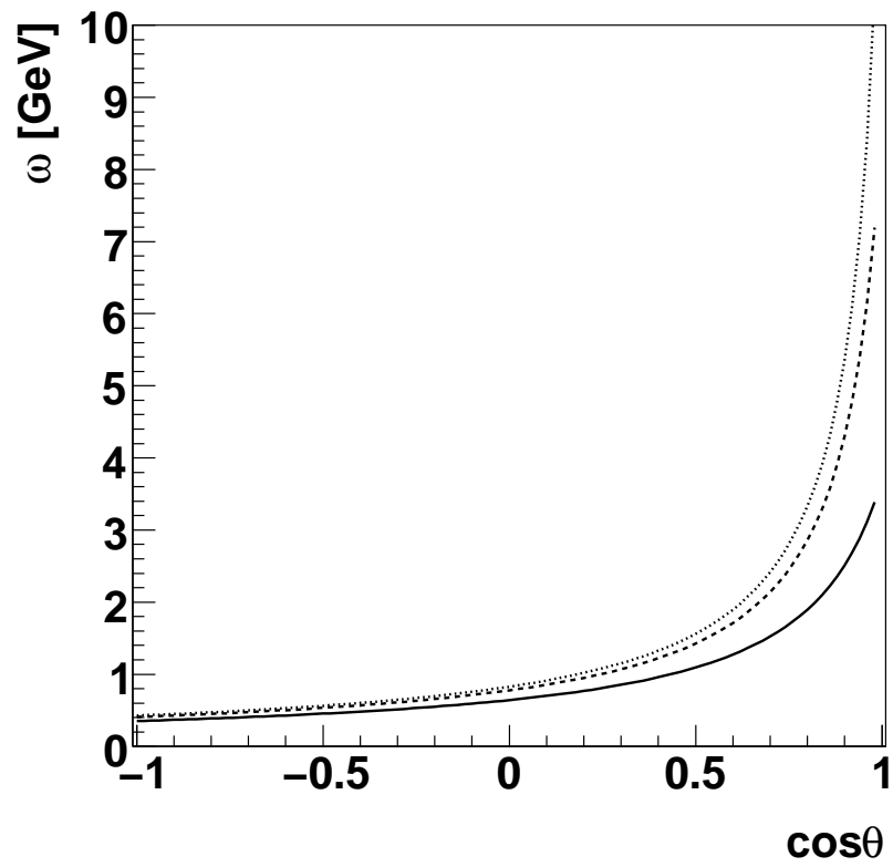
FIG. 2: Kinematical lines corresponding to protonium at rest in the plane \omega versus \cos\theta , for three values of the incident energy: E=5, 10 and 15 GeV, solid, dashed and dotted lines, respectively.
