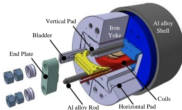
Fig. 1. SMC structure and main magnet components
