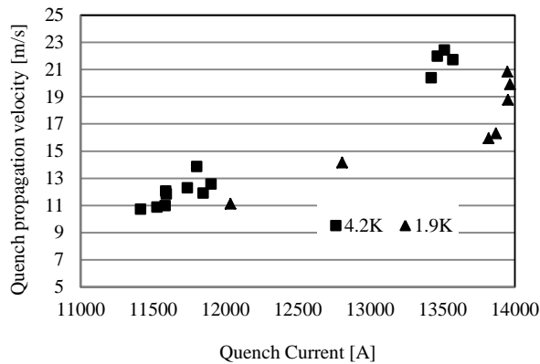
Fig. 4. Quenches propagation velocity calculated for quenches detected between Vtap 72 and 102, during training of SMC3.
