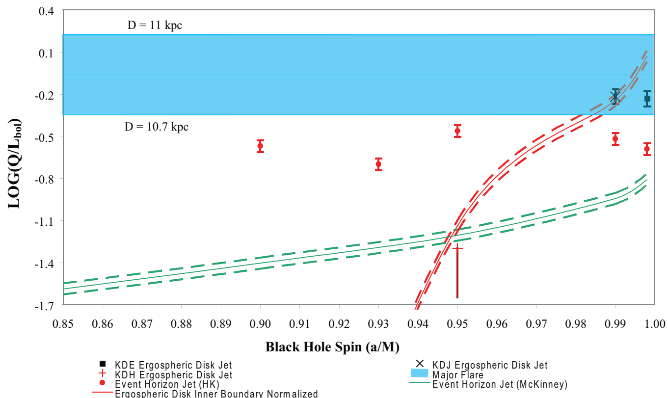
Fig. 5.— The logarithm of "jet power/ L_{\text{bol}} " in the numerical simulations compared to \log[\langle Q \rangle / \langle L_{\text{bol}} \rangle] for major flares in GRS 1915+105 based on Figure 4. The limited range of 10.7 \text{ kpc} < D < 11 \text{ kpc} indicated by the blue band, is the range of distance for which GRS 1915+105 can be considered a scaled down FR II quasar. The error bars and the range of uncertainty on the curves (the dashed curves) are based on the spread in Equation (5)
