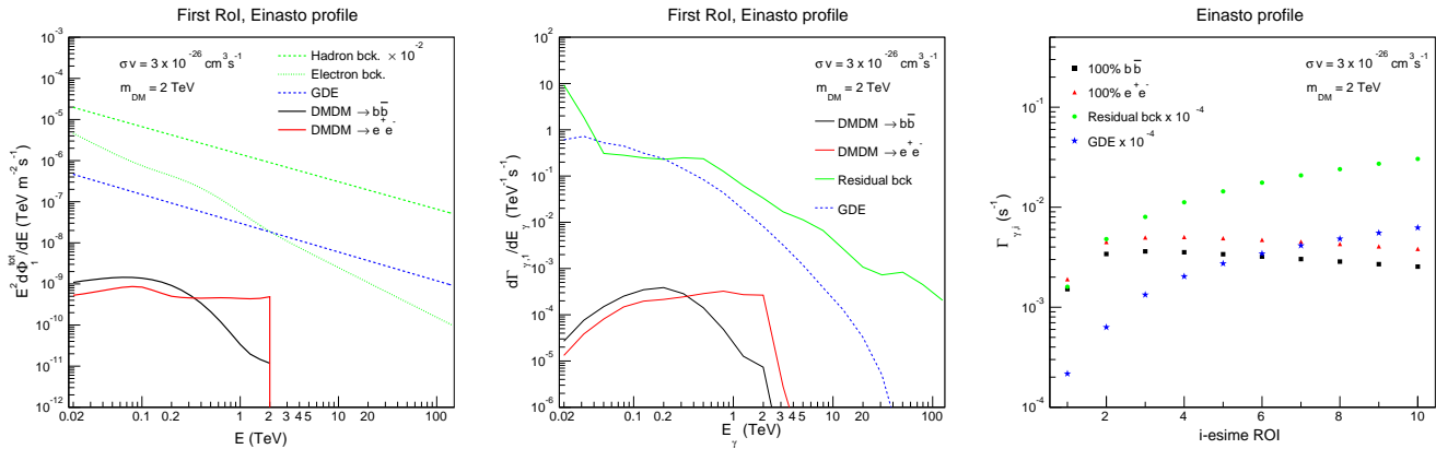
FIG. 2: Spectral and spatial morphology of typical DM signals together with the irreducible backgrounds. Left panel: Expected DM differential fluxes in the first RoI, considering 2 TeV thermal DM candidates annihilating into b\bar{b} (black solid line) and e^+e^- (red solid line) primary channels. For a sake of illustration, we show a spectrum for the CR hadrons (protons + nuclei) background (dashed green line) multiplied by a rejection factor \epsilon = 10^{-2} and a log-normal distribution for the electron spectrum (green dotted line) without rejection factor ( \epsilon_e = 1 ). The parametrizations of the irreducible backgrounds are given in Tab. 3 of Ref. [42]. Notice that the energy E in the y -axis, refers to the “true” energy of the particle which initiates the shower. The GDE flux detected by Fermi-LAT extrapolated at high energy is also shown as dashed blue line. Central panel: Expected differential count rate in the first RoI considering 2 TeV DM candidates with thermal cross section into b\bar{b} (black solid line) and e^+e^- (red solid line) primary channels. The most up-to-date CR background from a CTA Monte Carlo simulation (solid green line) and the GDE (dashed blue line) detected by Fermi-LAT in the same region are also presented for the sake of comparison. Right panel: Expected total rate summed over all energy bins in the i -esime RoI and for the same benchmark DM candidates (red filled triangle for annihilating DM into e^+e^- pairs, black filled square for b\bar{b} primary channel). The irreducible CR hadrons background in the i -esime RoI is identified as green filled circles, while our “extreme” isotropic GDE as blue-filled stars. See the text for further details.
