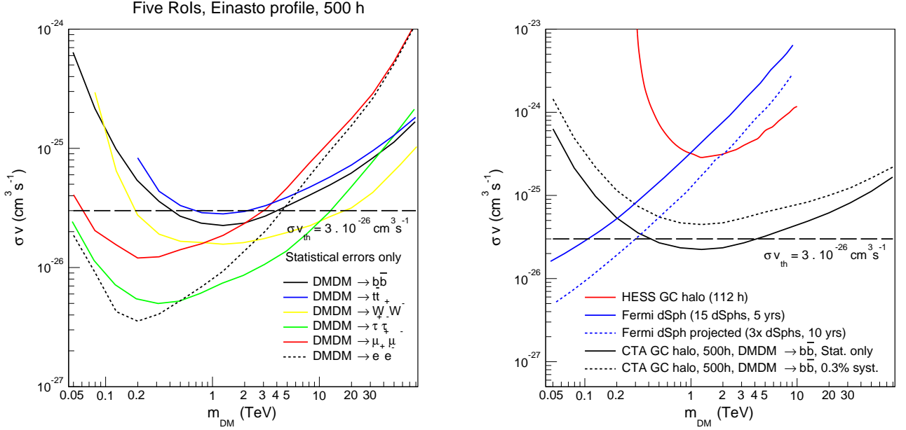
FIG. 4: Unless otherwise stated, the most optimist limits in the (m_{\text{DM}}, \langle\sigma v\rangle) plane in which neither the systematic uncertainties in the datasets nor the GDE are taken into account. Left panel: CTA sensitivity to DM annihilation for various primary channels (DM DM \rightarrow b\bar{b} in black, t\bar{t} in blue, W^+W^- in yellow, \tau^+\tau^- in green, \mu^+\mu^- in red and e^+e^- in dashed black) together with the reference value of the thermal cross section (long-dashed black line). The sensitivity is computed for a 500 h flat exposure over the five RoIs used in our analysis assuming a 100% branching ratio in each annihilation channel. Right panel: CTA sensitivity to DM annihilation for the DM DM \rightarrow b\bar{b} channel (black line) compared to the most constraining limits to date. In particular, we report the H.E.S.S. limit for 112h of observations of the GC region (solid red line) and the Fermi-LAT limit coming from 5 years of observations of 15 dSphs (solid blue line). An estimate of the projected sensitivity of Fermi-LAT for 45 dSphs and 10 years of observation time is also shown (dotted blue line). For a sake of comparison, we also report the CTA sensitivity assuming a reasonable 0.3% of systematics (dashed black line). See the text for further details.
