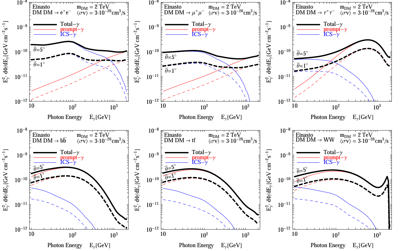
FIG. 1: Several example of \gamma -rays fluxes for 2 TeV DM candidates annihilating with thermal cross section ( \langle\sigma v\rangle = 3 \times 10^{-26} \text{ cm}^3/\text{s} ) into leptonic channels (first row) and hadronic ones (second row). In all plots, the different hashing shows the predicted signal in two benchmark RoIs with apertures \theta_1 (dotted line), and \theta_5 (solid line). The red, blue and thick black lines denote instead the spectral features of the prompt, ICSs and total fluxes respectively. See the text for further details.
