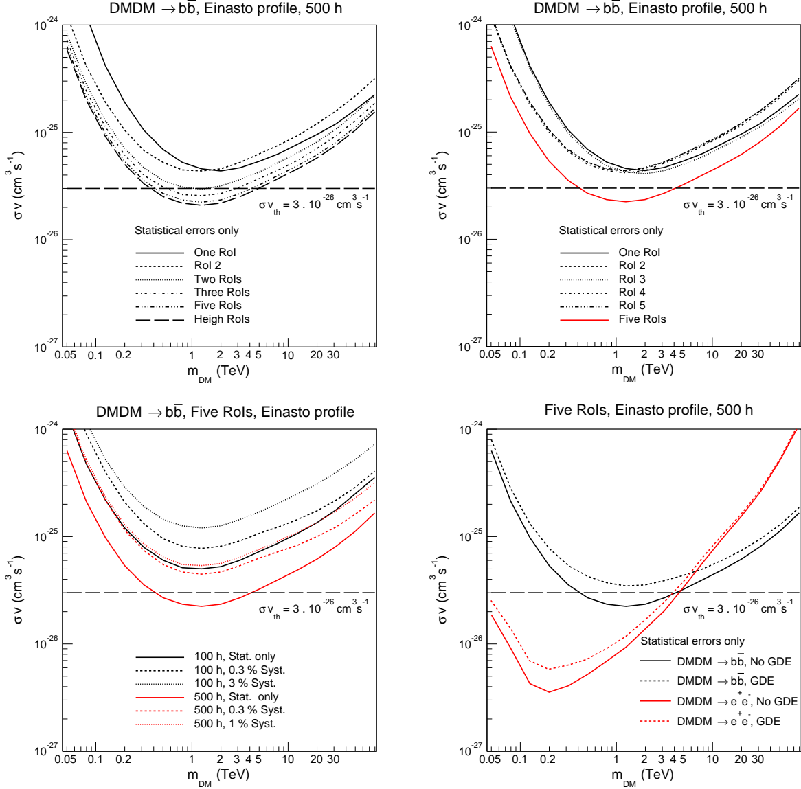
FIG. 3: CTA sensitivity to DM annihilation in the (m_{\text{DM}}, \langle\sigma v\rangle) plane. Unless otherwise stated, our morphological analysis employs five adjacent RoIs, the exposure in each RoIs is 500 h, the energy threshold is 30 GeV and only the statistical uncertainties are taken into account. Upper-left panel : Improvement of the CTA sensitivity for the DM \text{DM} \rightarrow \bar{b}b channel due to our multi-bin morphological method (two, three, five and eight RoIs) compared to the case where only the energy spectral information either in the first (solid black line) or in the second (dashed black line) RoI is taken into account. Upper-right panel : CTA sensitivity for the DM \text{DM} \rightarrow \bar{b}b channel when only the spectral information in the individual RoIs (RoI 1 to RoI 5) is considered. For a sake of comparison, we also show how our multi-bin morphological method (solid red line) ameliorates the CTA sensitivity. Bottom-left panel : Degradation of the CTA sensitivity for annihilating DM into \bar{b}b pairs due to possible systematic errors in the rich observational datasets. Observation times of 100 h (black lines) and 500 h (red lines) assuming different values of systematics: 0.3% (dashed lines), 3% (dotted lines), only statistical fluctuations (solid lines) are taken into account. Bottom-right panel : Impact of an “extreme” GDE added on top of the CR background, on the CTA sensitivity. The sensitivity is shown for annihilating DM into \bar{b}b (back lines) and e^+e^- (red lines) pairs with (dotted lines) and without (solid lines) the irreducible GDE background. See the text for further details.
