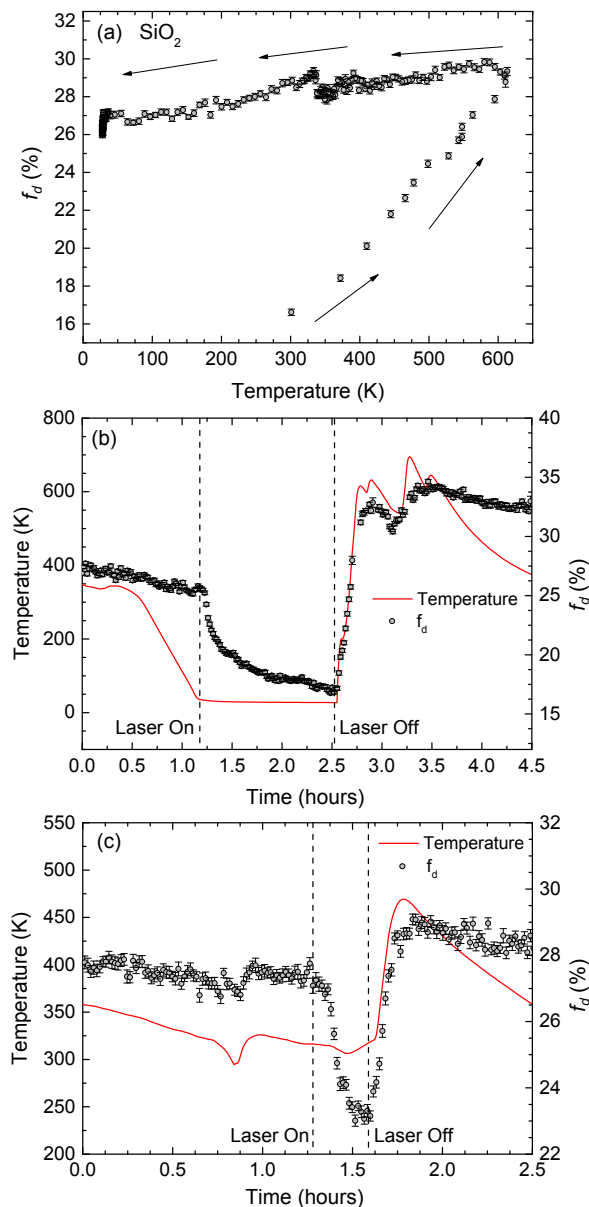
FIG. 8. (a) Delayed fraction ( f_d ) (filled circles) measured as a function of temperature for an \text{SiO}_2 sample as it is heated. Each point represents the average f_d value over a 30 second period. (b) Effect of cooling and laser irradiation on the delayed fraction, and (c) laser irradiation at room temperature following heating to \sim 600 K. In (b) and (c) the sample temperature is indicated by the solid (red) lines.
