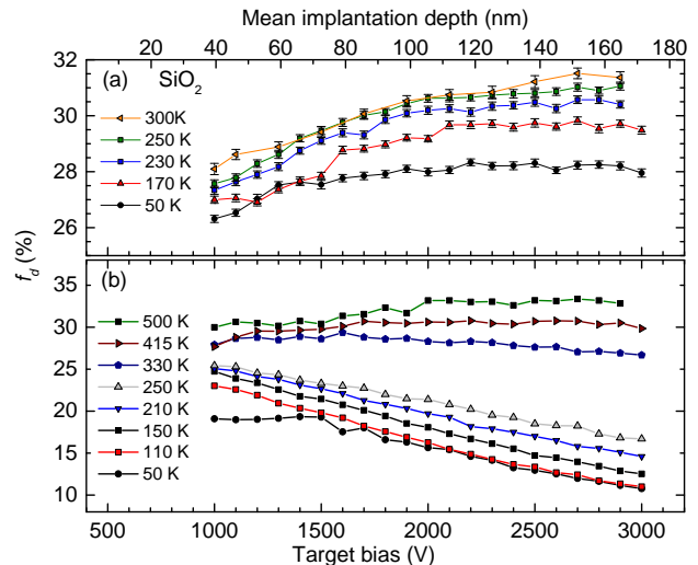
FIG. 9. f_d versus target bias at various temperatures for a \text{SiO}_2 sample with (b) and without (a) prior UV laser irradiation. The top axis indicates the mean implantation depth of the positrons. The irradiation and heating sequence is explained in the text. Error bars are not shown in (b) but are a similar size to those in (a).
