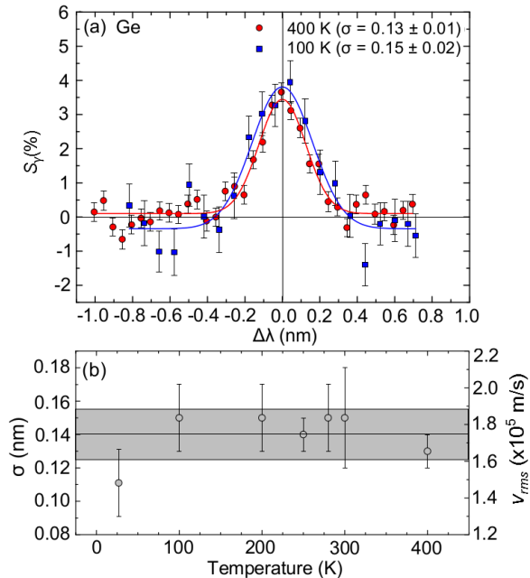
FIG. 14. Doppler spectroscopy of Ps emitted from single crystal Ge(100). (a) Doppler broadened line-shapes measured at 400 K and 100 K. (b) Values of \sigma obtained from linewidth measurements conducted at different sample temperatures. The gray band indicates the mean value of \sigma \pm 1 standard deviation ( 0.140 \pm 0.015 nm), and the corresponding RMS velocities. The positron beam energy was 0.65 keV for the data shown in (a) and 0.5 keV for the data in (b).
