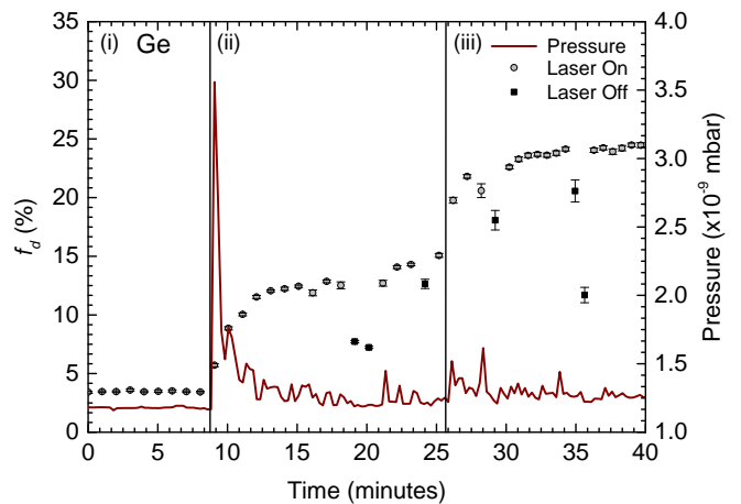
FIG. 13. Laser irradiation of a cold and contaminated Ge sample (the sample was kept at 27 K for \sim 12 hours) and its effect on ( f_d ). Different laser fluences were tested, as indicated by the numbered regions ((i) = laser off, (ii) = 10 mJ/cm 2 , (iii) = 24 mJ/cm 2 ). The square points were recorded with the photoemission laser temporarily blocked.
