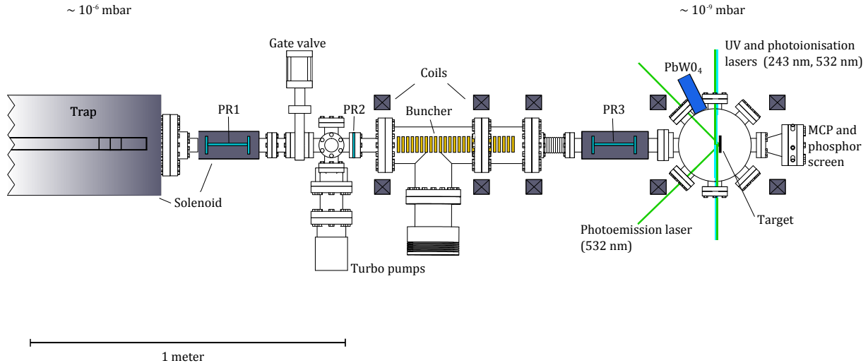
FIG. 2. Schematic layout of the positron beam following the two-stage buffer gas trap. The ^{22}\text{Na} source and slow positron beam that precedes the trap are described in Ref. 43 . Differential pumping is achieved using two 8 mm diameter tubes located inside solenoids (PR1 & PR3), and a 10 mm aperture (PR2) as indicated in the figure. Positrons are ejected from the trap with a 30 ns time width (FWHM) and are further bunched in time by a pulsed parabolic potential to a width of \sim 6 ns (FWHM) at the target. The configuration shown yields a pressure of \sim 10^{-9} mbar in the main target chamber. The cold head was mounted on an xyz manipulator and could be moved entirely out of the beam path, allowing the positron beam profile to be recorded on an imaging micro-channel plate (MCP) detector and phosphor screen assembly. The \text{PbWO}_4 scintillator is coupled to a PMT and oscilloscope in order to perform SSPALS 51 .
