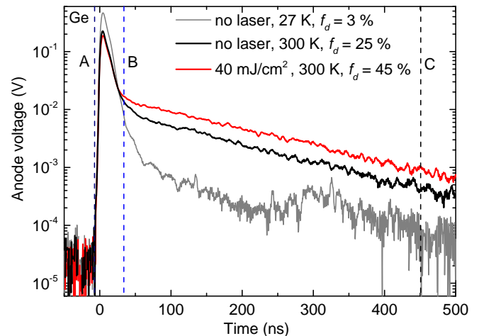
FIG. 1. Single-shot lifetime spectra measured with a Ge target, with and without a 532 nm photoemission laser, at 300 K and 27 K. The dashed vertical lines represent the time windows A , B and C . Each spectrum is the average of 100 individual shots.
