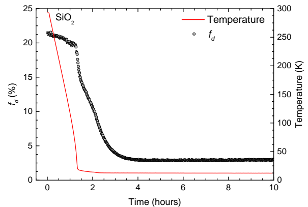
FIG. 4. Delayed fraction ( f_d ) from cooled mesoporous SiO 2 measured in the high-pressure ( 2 \times 10^{-6} mBar) chamber. The delayed fraction error bars ( \pm 0.1 %) are not shown.
