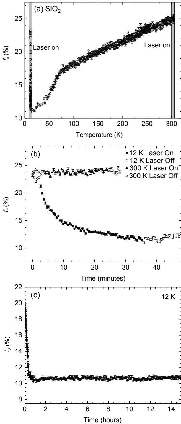
FIG. 7. (a) Delayed fraction ( f_d ) measured as a function of temperature for an \text{SiO}_2 sample irradiated with UV light pulses applied at 10 Hz. (b) Data from (a) plotted against time for laser irradiation at 12 and 300 K, as indicated in the legend. (c) Long-term stability of laser-induced paramagnetic centers. The sample remains cold ( \sim 12 K) following irradiation.
