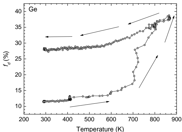
FIG. 10. Thermal desorption of Cl and concomitant increase in f_d , measured from single crystal Ge after insertion into the vacuum system. The measured temperatures above 700 K are inaccurate, as explained in the text. Each point represents the average f_d value over a 30 second period.
