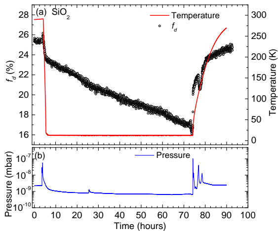
FIG. 5. (a) Delayed fraction ( f_d ) from cooled \text{SiO}_2 measured in the low-pressure ( 10^{-9} mBar) chamber. (b) Pressure in the target chamber associated with the cooling and heating cycle of (a).
