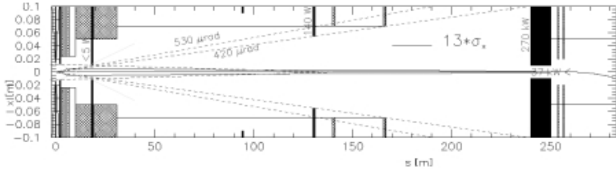
Fig. 5: Final transformer horizontal layout, with beamstrahlung average deposited power on collimators.
