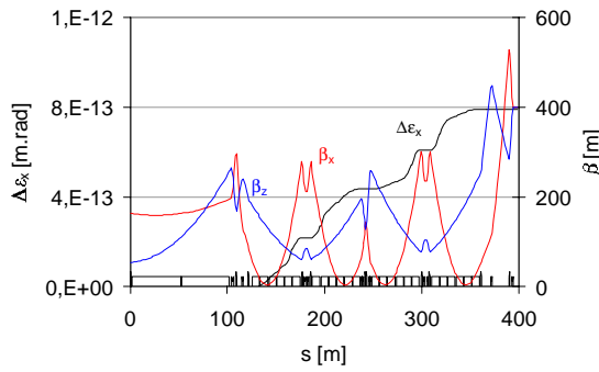
Fig. 3: Optics functions and emittance growth (at 400 GeV) for the BDS ARC.
