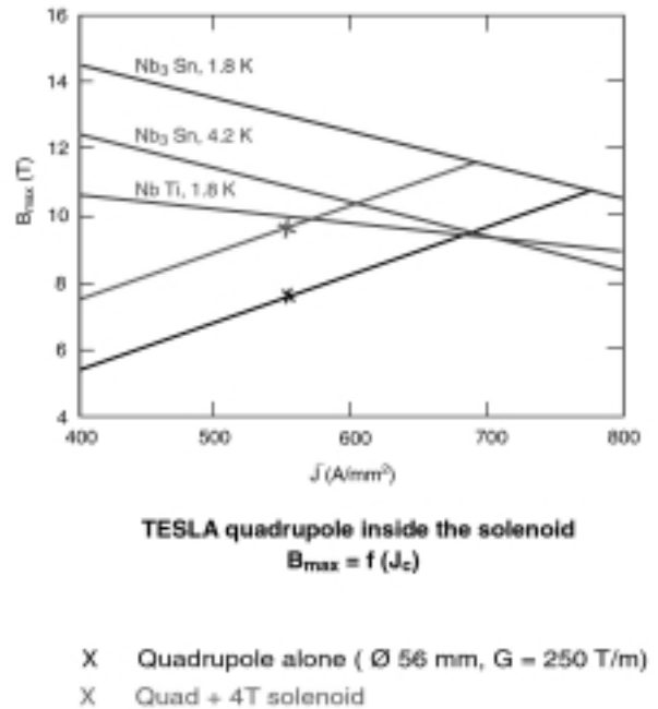
Fig.6: Superconducting quadrupole lines of charges compared to critical limits [5].
