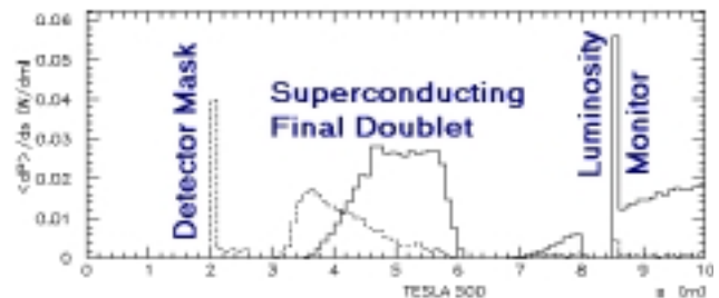
Fig.10: Average power , in units of W/dm, deposited by the radiative Bhabhas (solid) and e+e- pairs (dashed) in the interaction region (IP at s=0 ).
