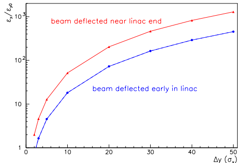
Figure 1: Relative increase in vertical emittance at the end of the linac for a mis-steered beam as a function of oscillation amplitude in units of rms beam size, simulated by the code PLACET [15]. Shown are the results of a bunch deflection after 10% and 90% of the full linac length.
