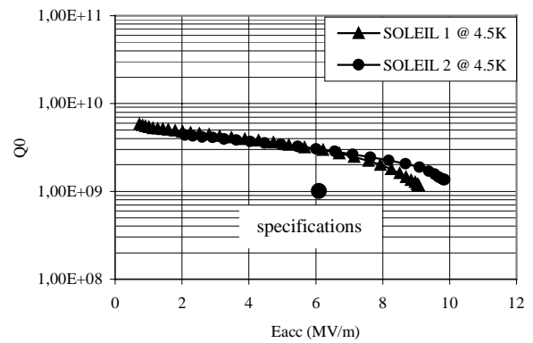
Figure 3: Q_0 versus the accelerating field curves of the two SOLEIL cavities at 4.5 K and 2.5 K.
