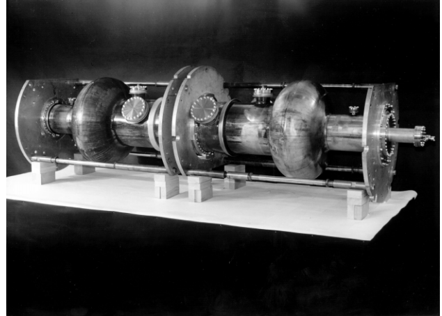
Figure 2: the two copper cavities after Nb deposition
