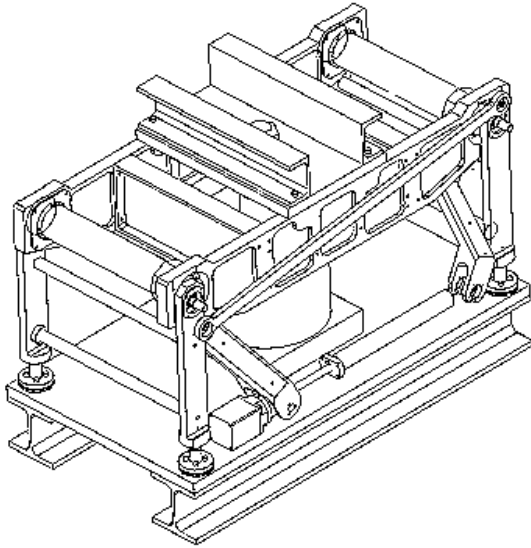
Figure 6: The tuning system of the cavities on its room temperature test stand. In the cryomodule, the four legs are fixed on the helium tank.
