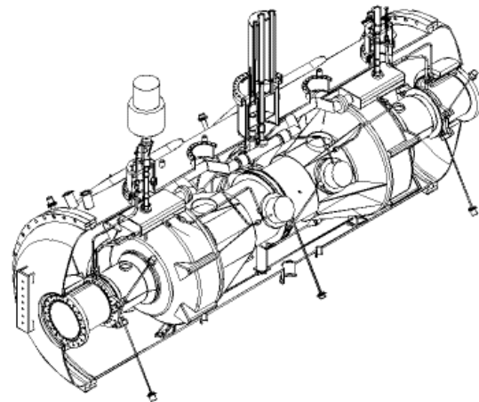
Figure 1: View of the cryomodule with the two helium tanks containing the cavities. (Tuning systems and power couplers are not represented).
