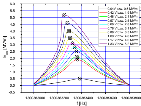
Fig. 7: Measurement of the cavity resonance curve (gradient vs. frequency) for increasing input power.
