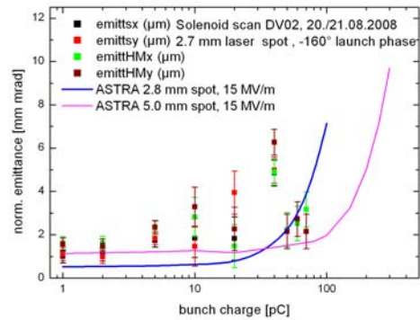
Fig. 16: Normalized transverse emittance as function of bunch charge for -160^\circ laser phase and 2.7 mm laser spot, as well as comparison with ASTRA simulation (15 MV/m peak field, 2.8 mm and 5 mm circular flat top laser spot, optimized phase and cathode position).
