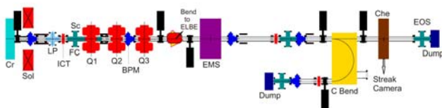
Fig. 10: Layout of the diagnostic beamline.
