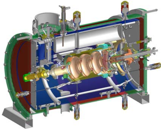
Fig. 1: Design of the SRF Gun cryomodule.
