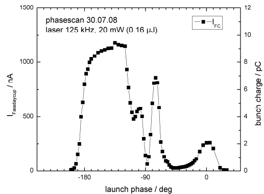
Fig. 11: Schottky scan at 125 kHz and 20 mW.
