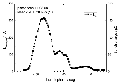
Fig. 12: Schottky scan at 2 kHz and 20 mW.
