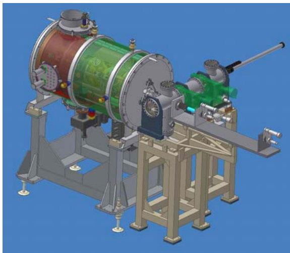
Fig. 3: Design of the photo cathode transfer system.
