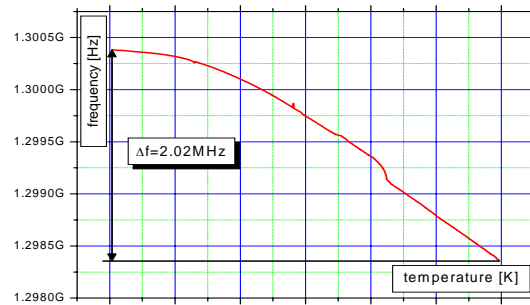
Fig. 4: Cool-down curve showing the cavity resonance frequency versus temperature.
