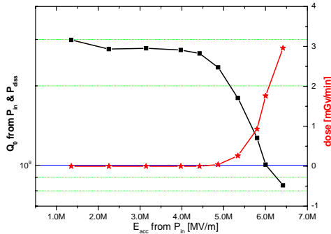
Fig. 6: Quality factor Q_0 versus acceleration gradient.
