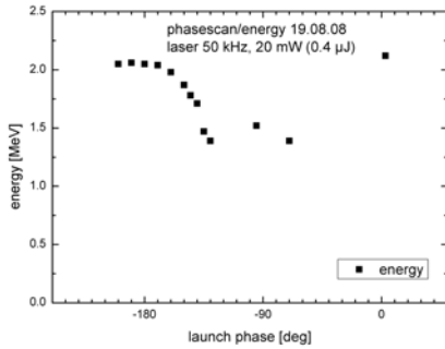
Fig. 13: Energy as a function of laser phase.
