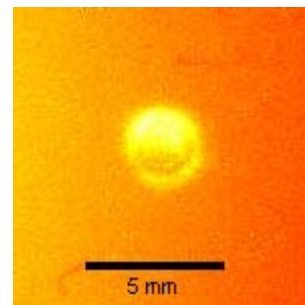
Fig. 8: CCD camera image of the laser spot at the virtual cathode. The spot diameter is 2.7 mm.
