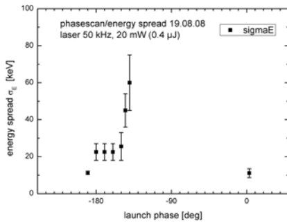
Fig. 14: The rms energy spread as function of laser phase.
