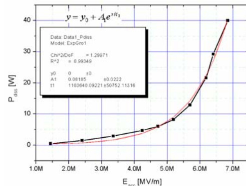
Fig. 5: RF power dissipation vs. gradient.
