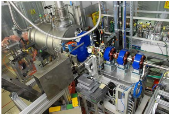
Fig. 2 : Photograph of the SRF gun in the ELBE accelerator hall.
