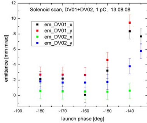
Fig. 15: Normalized transverse emittance as function of laser phase for 1 pC bunch charge.
