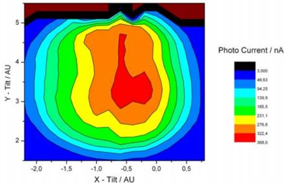
Fig. 9: Q.E. map of the Cs 2 Te photo cathode in the SRF gun. Photo current measured in the Faraday cup.
