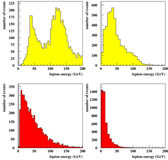
Figure 20: Distributions of the 2 muon energies (in GeV) in the events containing 2 same sign muons and at least 2 jets generated by the Standard Model background (lower curve), namely the W^\pm W^\mp , W^\pm Z^0 , Z^0 Z^0 , t\bar{t} , t\bar{b}/\bar{t}b and b\bar{b} production, and the SUSY signal (upper curve), for \lambda'_{211} = 0.05 , M_2 = 250\text{GeV} , m_0 = 200\text{GeV} , \tan\beta = 1.5 and \text{sign}(\mu) < 0 . The left plots represent the leading muon distributions and the right plots the second leading muon distributions. The numbers of events correspond to an integrated luminosity of \mathcal{L} = 10\text{fb}^{-1} .
