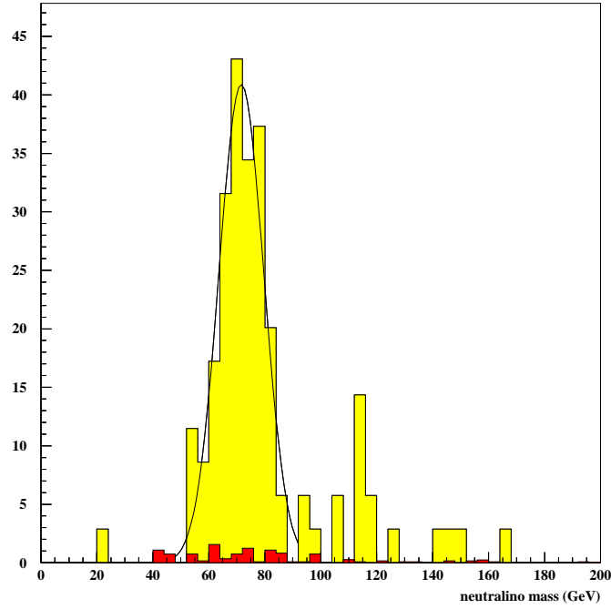
Figure 18: Distribution of the softer \mu + 2j invariant mass in the e + \mu + \mu + 2j + \nu events, for a luminosity of \mathcal{L} = 10fb^{-1} . The sum of the WZ , ZZ and t\bar{t} backgrounds is in black and the SUSY signal is in grey. The mSUGRA point taken for this figure is m_0 = 200GeV , M_2 = 150GeV , \tan\beta = 1.5 and sign(\mu) < 0 ( m_{\tilde{\chi}_1^0} = 77.7GeV ) and the considered \mathcal{R}_p coupling is \lambda'_{211} = 0.09 . The average reconstructed \tilde{\chi}_1^0 mass is 71 \pm 9 GeV .
