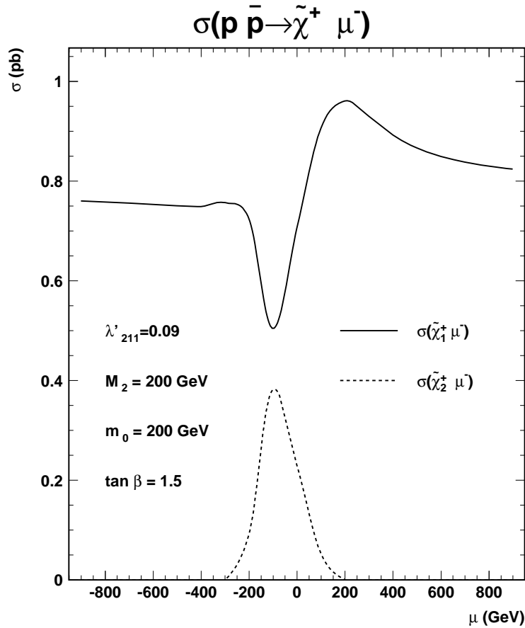
Figure 3: Cross sections (in pb) of the single chargino production p\bar{p} \rightarrow \tilde{\chi}_{1,2}^+ \mu^- as a function of the \mu parameter (in GeV) for \lambda'_{211} = 0.09 , M_2 = 200\text{GeV} , \tan\beta = 1.5 and m_0 = 200\text{GeV} at a center of mass energy of 2\text{TeV} .
