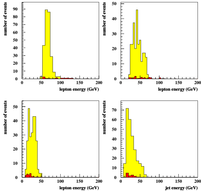
Figure 9: Energy distributions (in GeV) of the 3 leading charged leptons and the second leading jet in the events containing at least 3 charged leptons selected by applying cut 3 and produced by the Standard Model background (curve in black), namely the W^\pm Z^0 , Z^0 Z^0 and t\bar{t} production, and the SUSY signal (curve in grey), for \lambda'_{211} = 0.09 , M_2 = 150\text{GeV} , m_0 = 200\text{GeV} , \tan\beta = 1.5 and \text{sign}(\mu) < 0 . The upper left plot represents the leading lepton distribution, the upper right plot the second leading lepton distribution and the lower left plot the third leading lepton distribution. The numbers of events correspond to an integrated luminosity of \mathcal{L} = 10\text{fb}^{-1} .
