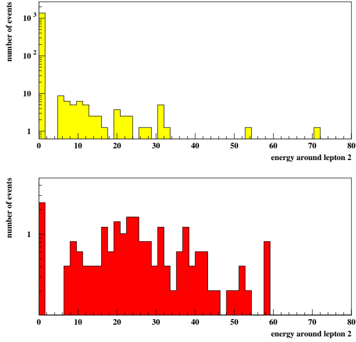
Figure 22: Distributions of the summed energies ( E , in GeV) of the jets being close to the second leading muon, namely the jets contained in the cone centered on the second leading muon and defined by \Delta R < 0.25 , in the like sign dimuons events selected by applying cut 2 and generated by the Standard Model background (lower curve), namely the W^\pm W^\mp , W^\pm Z^0 , Z^0 Z^0 , t\bar{t} , t\bar{b}/\bar{t}b and b\bar{b} production, and the SUSY signal (upper curve), for \lambda'_{211} = 0.05 , M_2 = 250\text{GeV} , m_0 = 200\text{GeV} , \tan\beta = 1.5 and \text{sign}(\mu) < 0 . These distributions were obtained after cut E < 2\text{GeV} , where E represents the summed energies of the jets being close to the leading muon, has been applied in these like sign dimuons events. The numbers of events correspond to an integrated luminosity of \mathcal{L} = 10\text{fb}^{-1} .
