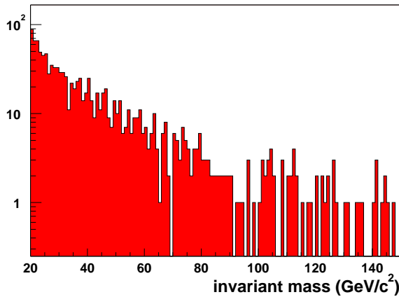
\mu\mu invariant mass
