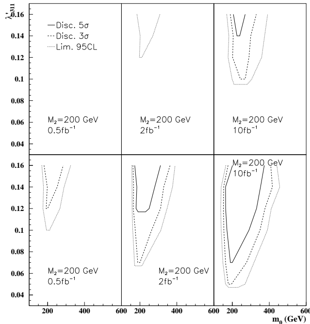
Figure 17: Discovery contours at 5\sigma (full line), 3\sigma (dashed line) and limit at 95% C.L. (dotted line) presented in the plane \lambda'_{311} versus the m_0 parameter, for \text{sign}(\mu) < 0 , \tan\beta = 1.5 , M_2 = 200\text{GeV} and different values of luminosity. The upper (lower) curves are obtained without (with) the reconstruction of the tau-jets.
