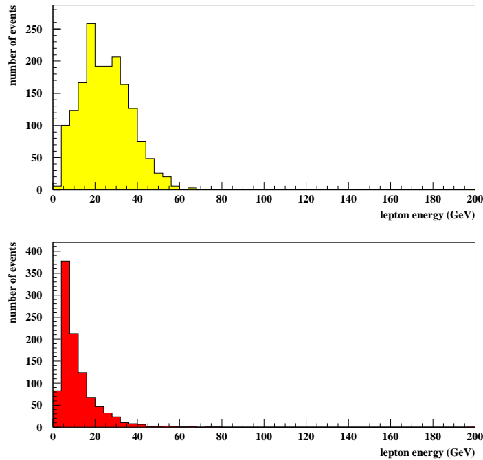
Figure 7: Distributions of the lowest lepton energy (in GeV) among the energies of the 3 leading leptons (electrons and muons) in the events containing at least 3 charged leptons and 2 jets generated by the Standard Model background (lower curve), namely the W^\pm Z^0 , Z^0 Z^0 and t\bar{t} production, and the SUSY signal (upper curve), for \lambda'_{211} = 0.09 , M_2 = 150\text{GeV} , m_0 = 200\text{GeV} , \tan\beta = 1.5 and \text{sign}(\mu) < 0 . The numbers of events correspond to an integrated luminosity of \mathcal{L} = 10\text{fb}^{-1} .
