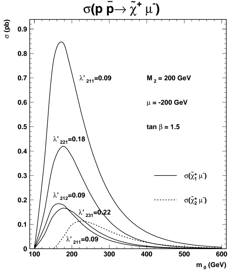
Figure 5: Cross sections (in pb) of the single chargino production p\bar{p} \rightarrow \tilde{\chi}_1^+ \mu^- as a function of the m_0 parameter (in GeV). The center of mass energy is taken at \sqrt{s} = 2\text{TeV} and \lambda'_{211} = 0.09 , M_2 = 200\text{GeV} , \tan\beta = 1.5 and \mu = -200\text{GeV} . The rates of the single \tilde{\chi}_1^+ production via the \mathcal{R}_p couplings \lambda'_{212} = 0.09 , \lambda'_{221} = 0.18 and \lambda'_{231} = 0.22 are also shown. The chosen values of the \mathcal{R}_p couplings correspond to the low-energy limits [4] for a squark mass of 100\text{GeV} .
