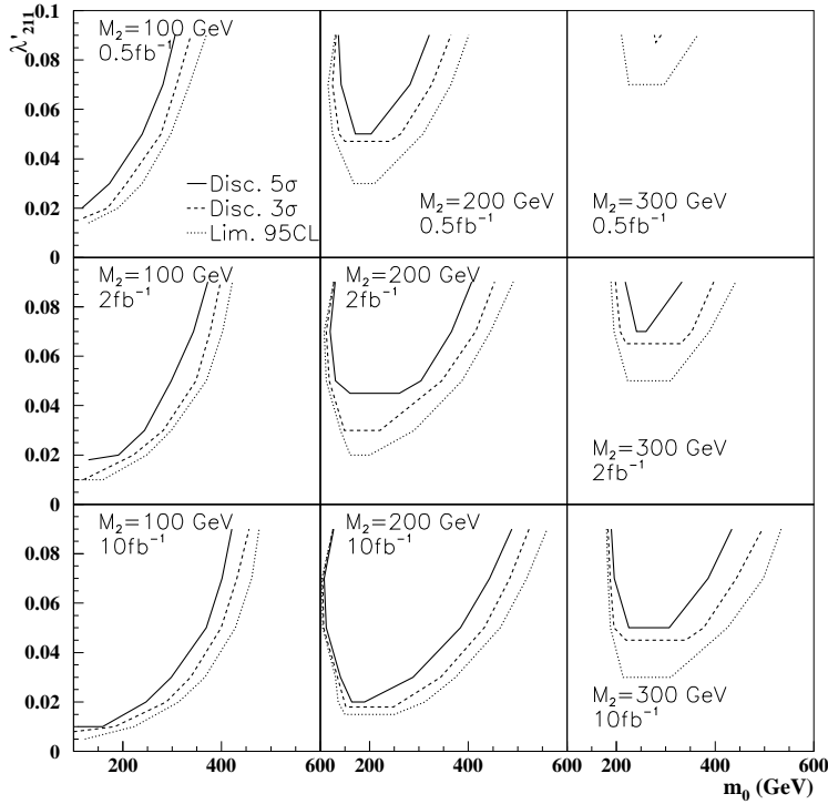
Figure 11: Discovery contours at 5\sigma (full line), 3\sigma (dashed line) and limit at 95% C.L. (dotted line) presented in the plane \lambda'_{211} versus the m_0 parameter, for \text{sign}(\mu) < 0 , \tan\beta = 1.5 and different values of M_2 and of luminosity.
