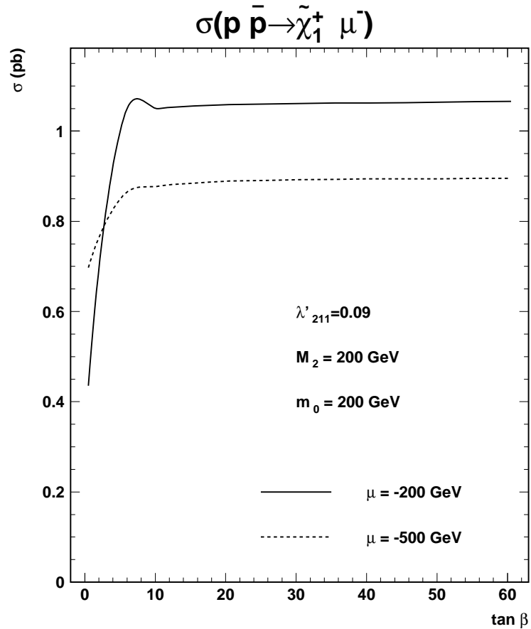
Figure 2: Cross sections (in pb) of the single chargino production p\bar{p} \rightarrow \tilde{\chi}_1^+ \mu^- at a center of mass energy of 2TeV as a function of the \tan\beta parameter for \lambda'_{211} = 0.09 , M_2 = 200\text{GeV} , m_0 = 200\text{GeV} and two values of the \mu parameter: \mu = -200\text{GeV} , -500\text{GeV} .
