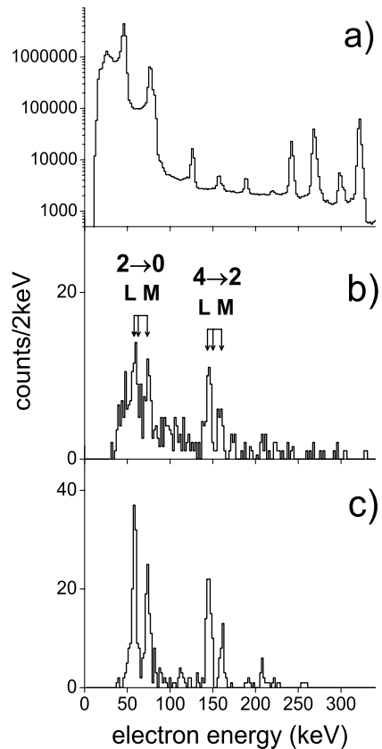
FIG. 1: (a): Spectrum of ^{133}\text{Ba} source, showing the detector response on a logarithmic scale. (b): Experimental conversion electron spectrum (corrected for the contribution from random coincidences) tagged by the characteristic \alpha -decay of ^{226}\text{U} . In this spectrum the energies are not corrected for Doppler shift. Transitions in the ground state band are identified. (c): Simulated spectrum for ^{226}\text{U} as described in the text.
