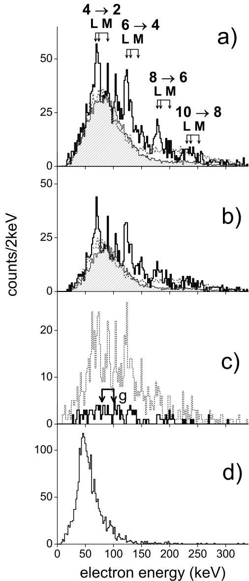
FIG. 2: (a): The experimental conversion electron spectrum tagged by ^{254}\text{No} recoils, corresponding to any number of electrons detected in SACRED (solid bold line). In this spectrum the energies are not corrected for Doppler shift. The lowest transitions in the ground state band are identified. Also shown are the simulated spectra as described in the text for g_K = 0 (hashed area with solid line border) and for g_K - g_R = 0 (dashed line). (b): as (a) except that experiment and simulation correspond to the detection of a single electron. (c): Spectrum of second electron in coincidence with a selected region (labelled 'g') of energy for the first electron, tagged by recoils (solid bold line). Also shown is the experimental spectrum tagged by \alpha -decay for any number of electrons detected (dashed line). (d): electron spectrum taken in random coincidence.
