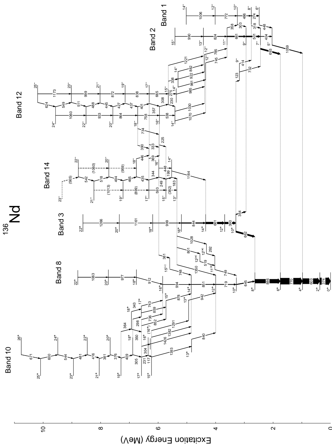
Fig. 2. Level scheme of ^{136}\text{Nd} deduced from the present work. The transition intensities are proportional to the width of the arrows. Transitions indicated by dashed lines are tentative.
