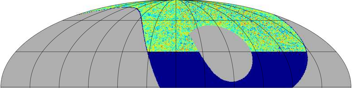
Fig. 1. Archeops CMB map (Galactic coordinates, centered on the Galactic anticenter, Northern hemisphere) in HEALPIX pixelisation (Gorski et al. 1998) with 15 arcmin. pixels and a 15 arcmin. Gaussian smoothing. The map is a two-photometers co-addition. The dark blue region is not included in the present analysis because of possible contamination by dust. The colors in the map range from -500 to 500 \mu\text{K}_{\text{CMB}} .
