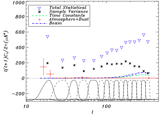
Fig. 3. Contamination by systematics : the Archeops CMB power spectrum statistical error bars (including noise and sample variance) are shown as the blue triangles. The large error bar in the first bin mainly comes from the high-pass filtering. A conservative upper-limit to contamination by dust and atmospheric signal is shown in red crosses, with a \ell different binning to enhance the low \ell side. Beam and time constants uncertainties are shown in dot-dashed blue and dashed green (see text). The 7% temperature calibration uncertainty is not shown here. The window functions are shown at the bottom of the figure.
