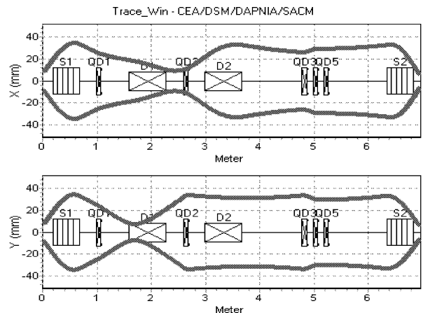
Figure 3: Ion envelopes in the LEBT.
