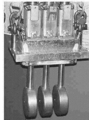
Figure 1: The hot model's girder with all three drift tubes fitted.
