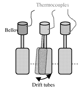
Figure 5: Measurement of the drift tube's misalignment influence on the bellows heating. Top: principle of the test; the central drift tube is shifted left or right and the temperature is measured on all three bellows (at different altitudes). Bottom: heating on all three bellows. The central bellow (rose curve) is the hotter, and the influence on adjacent bellow is sensible but smaller. Tests are performed at 25% of the nominal power.
