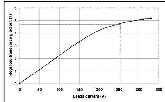
Figure 6: Integrated gradient measurement of the flooded quadrupole magnet for various currents. Effect of saturation is clearly shown.
