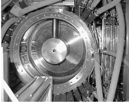
Figure 2: Inside view of the hot model tank with drift tubes fitted.
