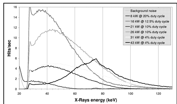
Figure 4: Measurement of the accelerating field using X-ray spectrometry method for different power levels.
