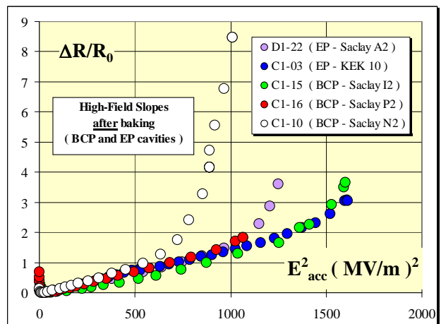
Figures 8: Residual Q_0 -slopes before and after baking (EP and BCP cavities)
