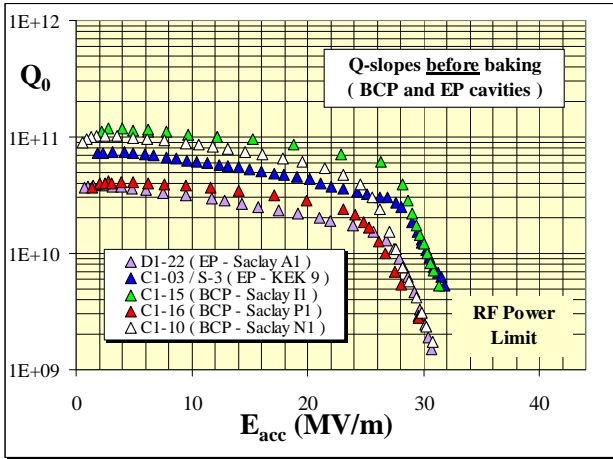
Figure 5: Q_0 -slope similarities before “in-situ” baking between EP and BCP cavities
