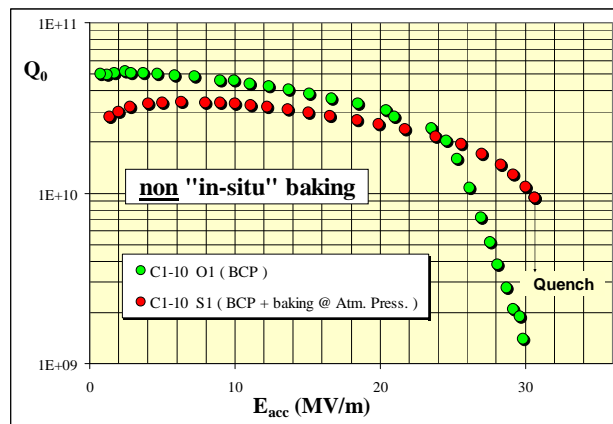
Figure 1: Q 0 -slope Improvement for BCP cavity by using a non “in-situ” baking.
