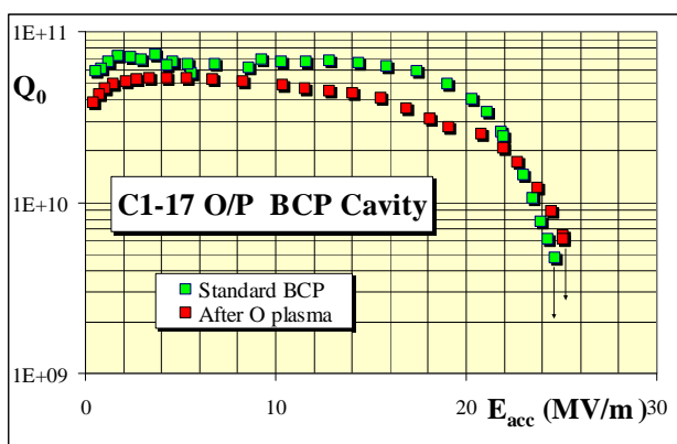
Figure 2: Q_0(E_{\text{acc}}) before and after \text{O}^+ plasma treatment
