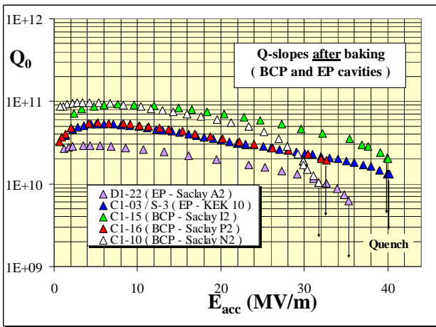
Figure 6: Q_0 -slope Improvement after baking
