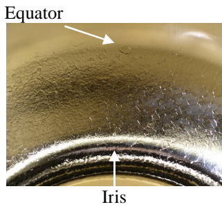
Figure 7a: Picture of the inner surface of C1-10 (residual Q-slope after baking)
