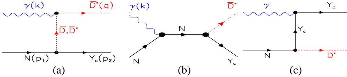
FIG. 1: The pole mechanisms for \gamma + N \rightarrow Y_c + \overline{D}^* .
