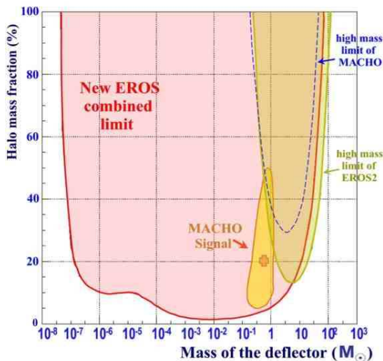
Fig. 1. Exclusion diagram (95% C.L.) on the halo mass fraction in the form of compact objects of mass M , for the standard halo model ( 410^{11} Solar masses inside 50 kpc), from all LMC and SMC EROS data. The thick line is the combined limit from all EROS sub-experiments. The dotted line indicates the high mass limit of the MACHO experiment, while the enclosed region, marked by an arrow, represents the signal reported by the MACHO experiment, and excluded by EROS. For MACHOs with mass between 10^{-6} and 3 solar masses, the EROS result shows that the MACHO contribution to the galactic halo is less than 10% (after Ref. [16])
