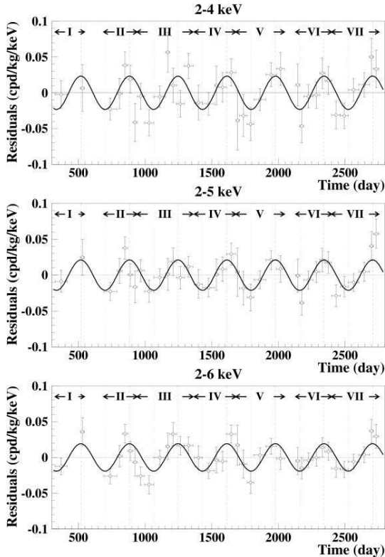
Fig. 4. Annual modulation amplitude reported by the DAMA experiment using a \sim 10^5 kg \times day data sample, recorded over a period of seven years. The statistical significance of the detected modulation is \sim 6.2 standard deviations (from Bernabei et al. Ref. [52])
