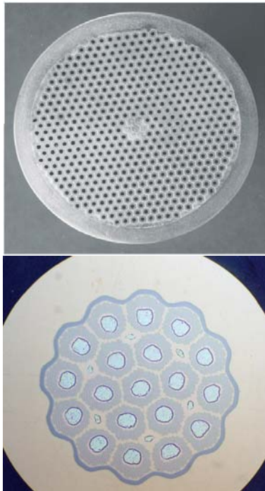
Fig. 2. Examples of \text{Nb}_3\text{Sn} wires developed in Europe for HEP applications: (a) binary- \text{Nb}_3\text{Sn} PIT wire produced by SMI (top); (b) ternary- (\text{NbTa})_3\text{Sn} internal-tin wires produced by Alstom/MSA (bottom). Both wires have 18-to-20 \mu\text{m} effective filament diameters.
