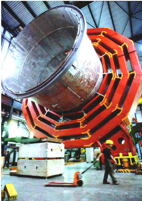
Fig. 2. View of the central barrel yoke ring equipped with the outer vacuum tank destined to house the superconducting coil.
