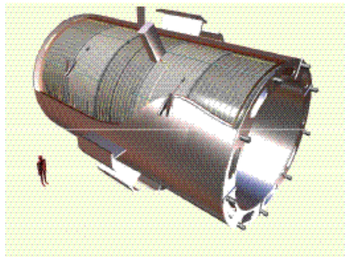
Fig. 4. Perspective view of the CMS coil inside the outer vacuum tank showing the five modules, the tie-bar suspension system, and the thermosiphon cooling circuits outside the mandrels.
