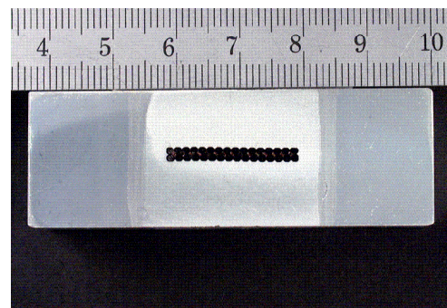
Fig. 5. Cross section of the CMS conductor. One can note the two alloy sections attached by Electron Beam welding to the pure aluminium insert comprising the 32-strand Rutherford cable.
