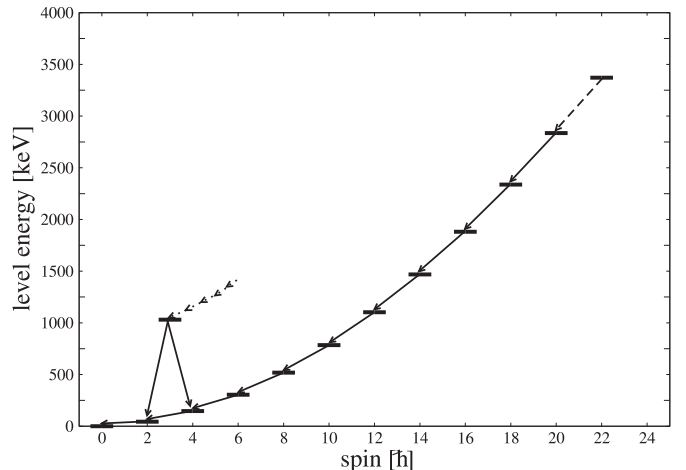
Figure 6. Yrast plot of ground-state band with suggested positioning of high energy lines. The assumed feeding pattern of the high-lying low-spin state is shown with dashed lines.
