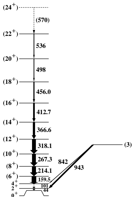
Figure 4. Proposed partial level scheme of ^{254}\text{No} (see 4.1 and 4.2).
