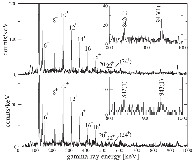
Figure 1. Upper panel: Recoil-gated \gamma -ray singles spectrum of ^{254}\text{No} . The rotational ground-state band transitions are labelled with their respective spin assignments. The inset displays an expansion of the spectrum showing the two prominent high-energy \gamma -ray peaks. Lower panel: Recoil-decay tagged \gamma -ray singles spectrum of ^{254}\text{No} . The search time was 180 seconds. Again, the inset shows the high-energy peaks.
