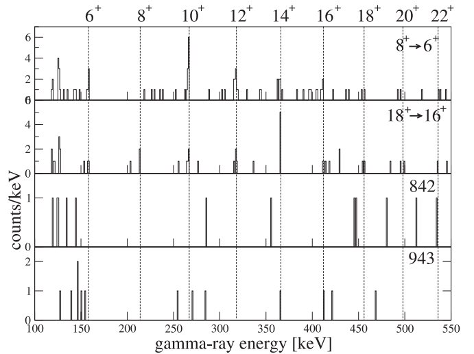
Figure 3. Example spectra projected from the recoil-gated \gamma - \gamma coincidence matrix. The labels in the upper right-hand corner indicate the transition or transition energy used as a gate. The upper two panels show spectra gated on ground-state band transitions, the lower two spectra gated on the high-energy transitions. Dotted lines indicate the positions of the ground-state band transitions.
