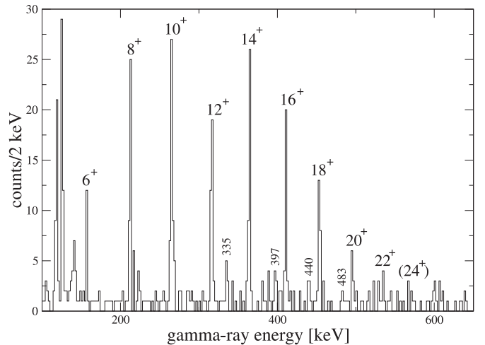
Figure 2. A sum of \gamma -ray spectra projected from the recoil-gated \gamma - \gamma coincidence matrix. The spectrum is a sum of spectra gated on ground-state band transitions from the 6^+ state up to the 18^+ state.
