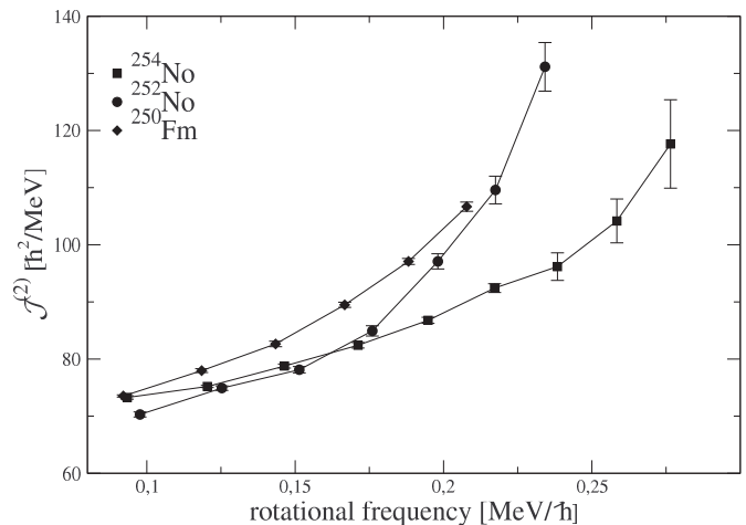
Figure 5. Dynamical moment of inertia \mathcal{J}^{(2)} against rotational frequency of the ground-state band of ^{254}\text{No} , compared with that of the N = 150 isotones ^{252}\text{No} [29] and ^{250}\text{Fm} [30].
