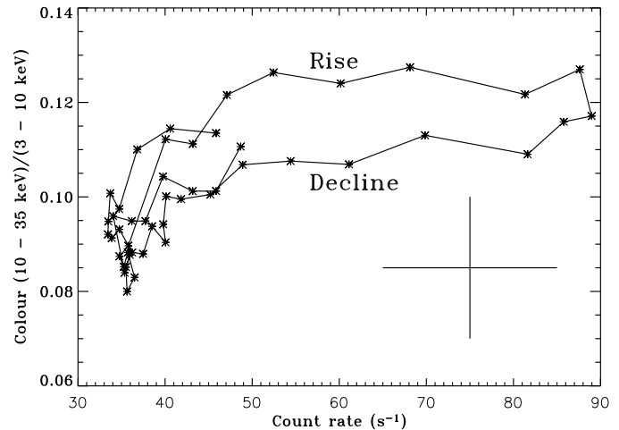
Fig. 4. The JEM-X colour-intensity diagram from the whole 100 ks observation. The colour was constructed from the 10–35 keV and 3–10 keV lightcurves. The maxima of the flares are in the right-hand edge of the plot, while the minima are in the left-hand edge. This confirms that the rising phases are harder than the declining phases. Each point is one time bin (10 s) and represents the averaged mean value from the 300 JEM-X flares; the cross shows the average standard deviation for the mean value of each individual point throughout the loop – this includes both the variability within each point and the error (i.e. it is not an error bar).
