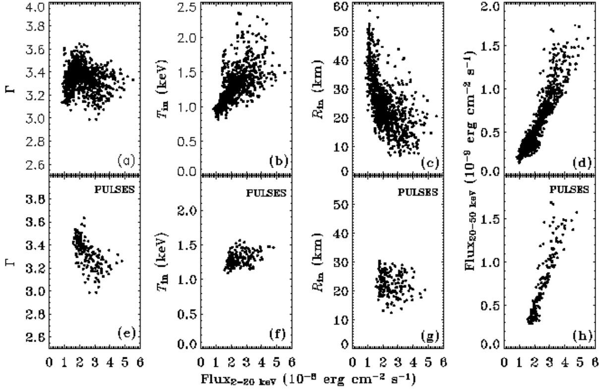
Fig. 8. Panels a–d show \Gamma , T_{\text{in}} , R_{\text{in}} and the 20–50 keV flux against the 2–20 keV flux from the whole set of the RXTE /PCA observations, while panels e–h show the same but only for the pulses.
