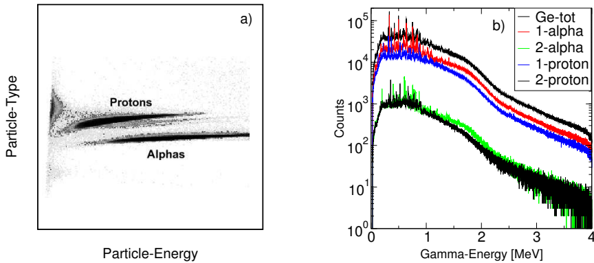
Fig. 1. a) Particle-type vs. Energy spectrum used for determining particle gates for channel selection purposes. b) Total projection Ge-spectra for the charged-particle channels, showing the presence of huge E2-bump for the \alpha -xn channels.
