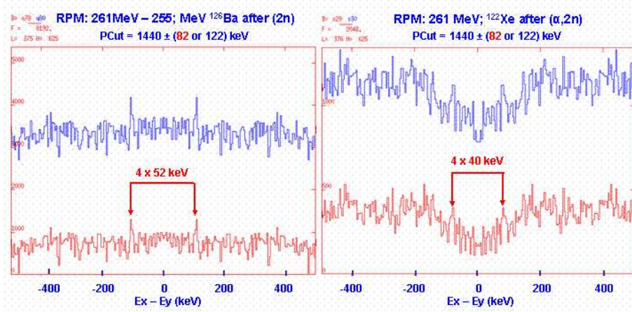
Fig. 2. a) The right panel shows the first results for the HD ridge structures observed by Rotational Plane Mapping in coincidence with \alpha -particles, presumably in ^{122}\text{Xe} as discussed in the text. It is compared to the similar results shown in the left panel, obtained by 2n reaction going to ^{126}\text{Ba} . The lower and upper spectra in both panels correspond to perpendicular cuts of (E_x + E_y)/2 = 1440 \pm 82\text{keV} , and (E_x + E_y)/2 = 1440 \pm 122\text{keV} , respectively.
